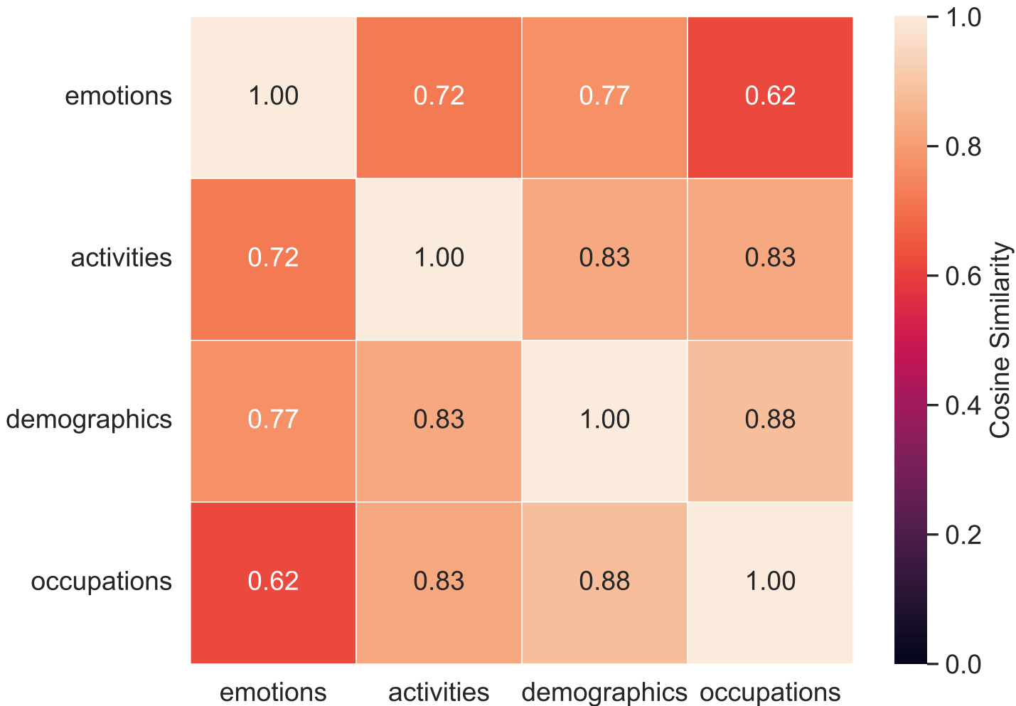
Cosine Similarity of Steering Vectors
