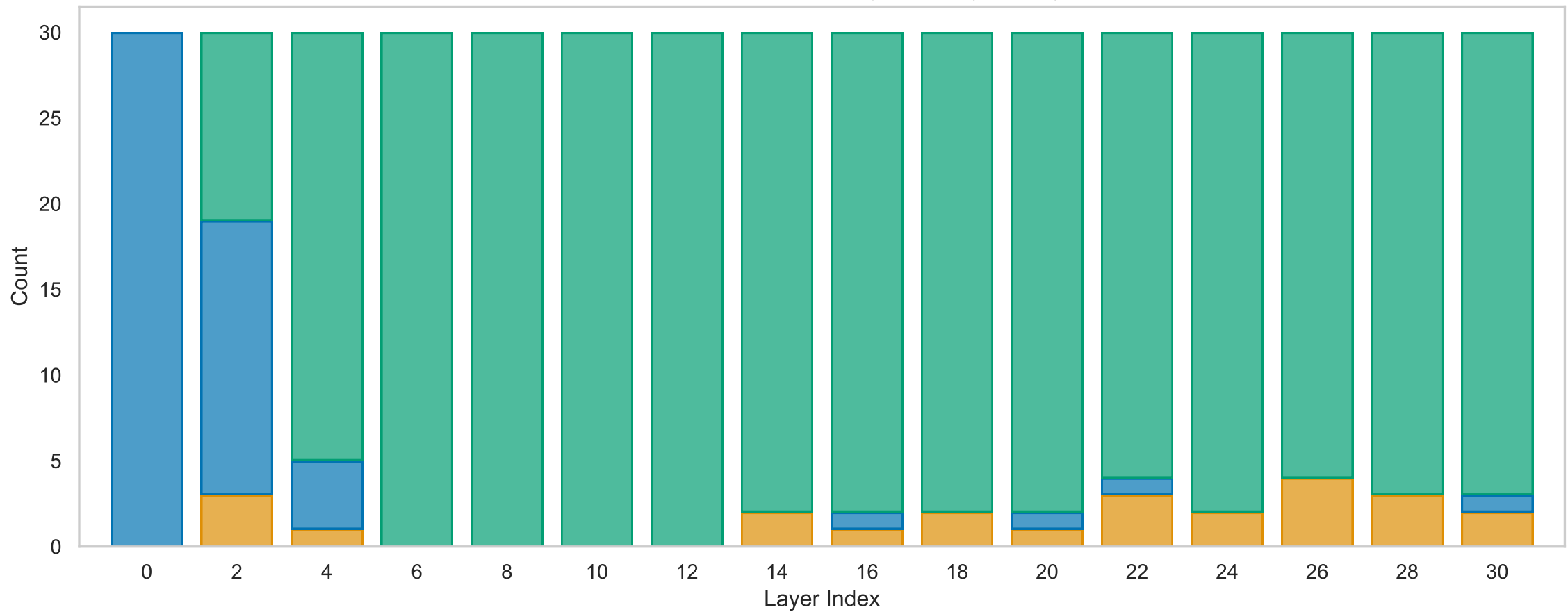
Stacked Label Counts per Layer Index (Positive)
