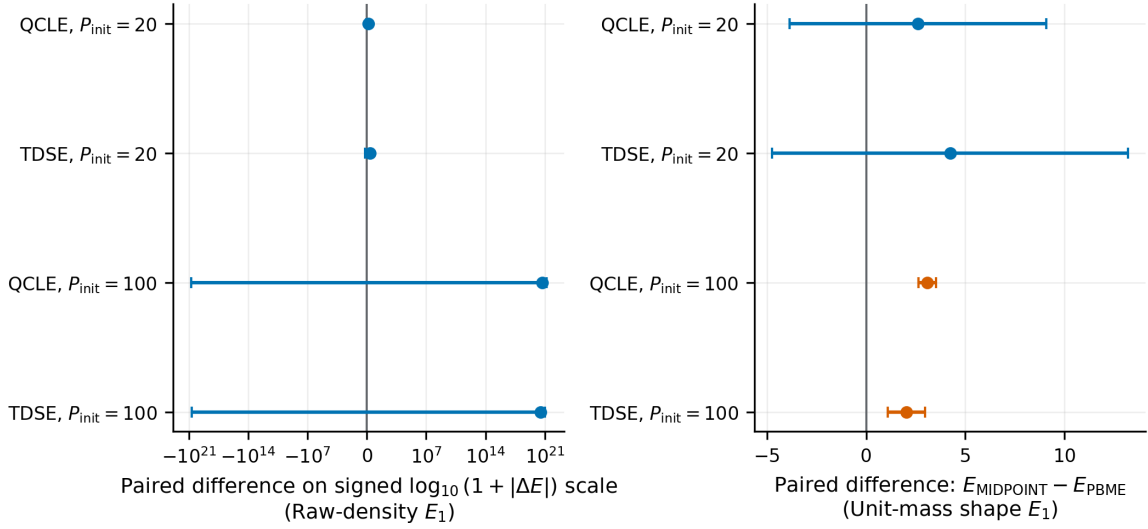
Figure 6.5: Four-seed paired MIDPOINT-minus-PBME differences for density E_1 errors against the matched TDSE and grid-QCLE references. Points are paired means and bars are two-sided Student- t 95% intervals with three degrees of freedom. Positive values mean that MIDPOINT has the larger error. The raw-density panel uses the signed display transform \text{sgn}(\Delta E) \log_{10}(1 + |\Delta E|) , whose tick labels show the corresponding untransformed magnitude; the shape panel uses unit-mass normalization and a linear axis. Shape agreement is therefore not used as conservation evidence.
