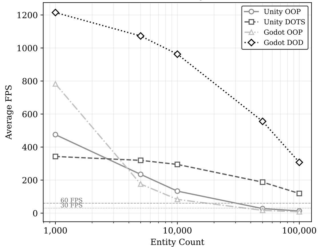
(b) FPS vs. Entity Count
