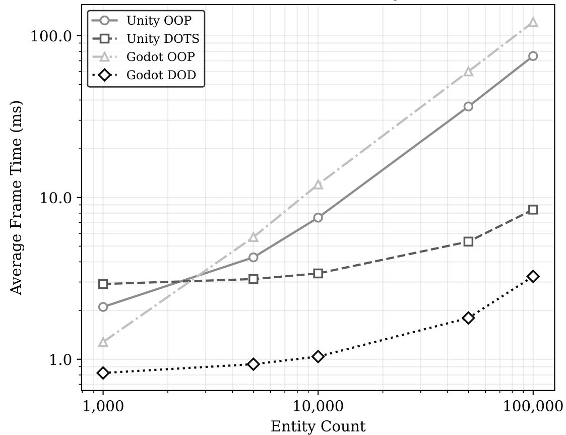
(a) Frame Time vs. Entity Count
