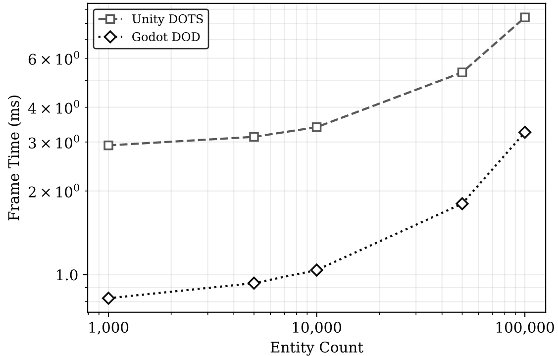
(b) Cross-Engine, DOD Level (Burst+ECS vs. C++ SoA)
