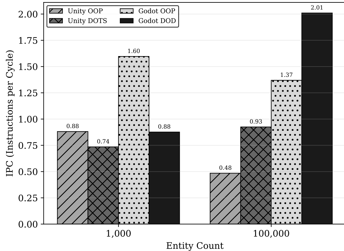
(a) IPC vs. Entity Count
