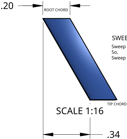
TOP PLANFORM VIEW
