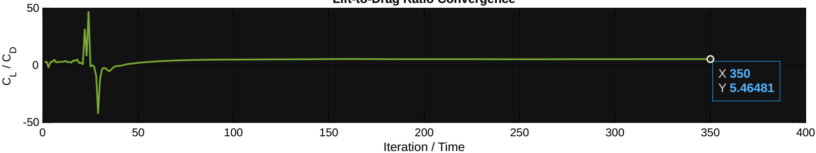
Lift-to-Drag Ratio Convergence
