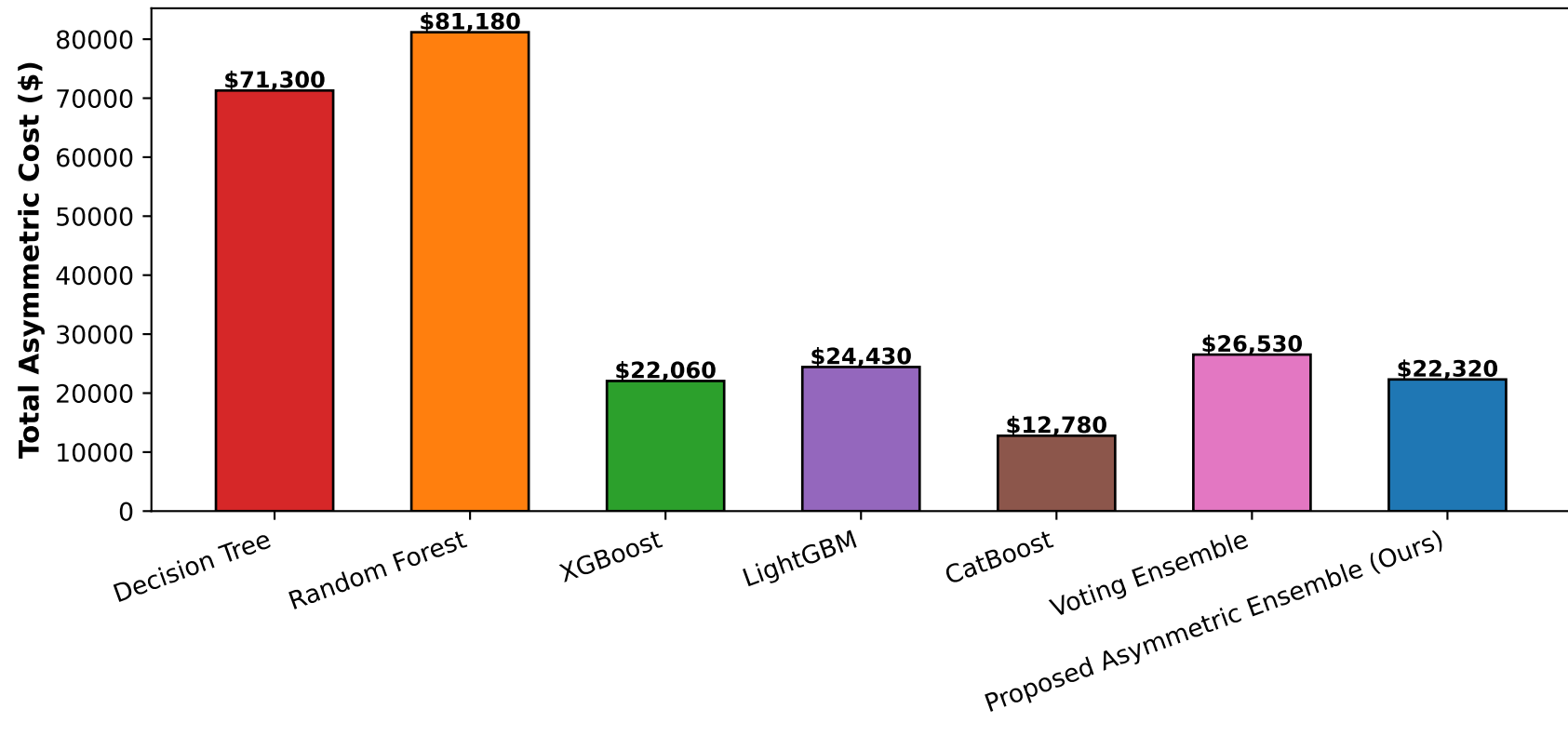
Asymmetric Cost Minimization Comparison ( C_{FP} = \$10 , C_{FN} = \$500 )
