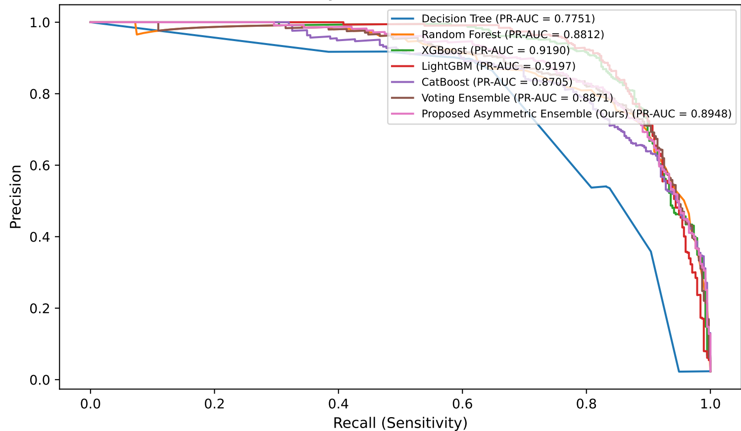
Precision-Recall Overlay Curves under Severe Class Imbalance
