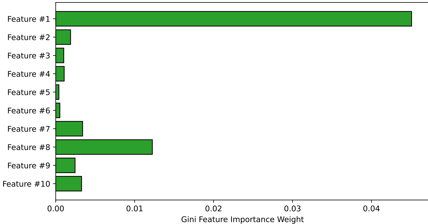
XGBoost Baseline Feature Importance Ranking
