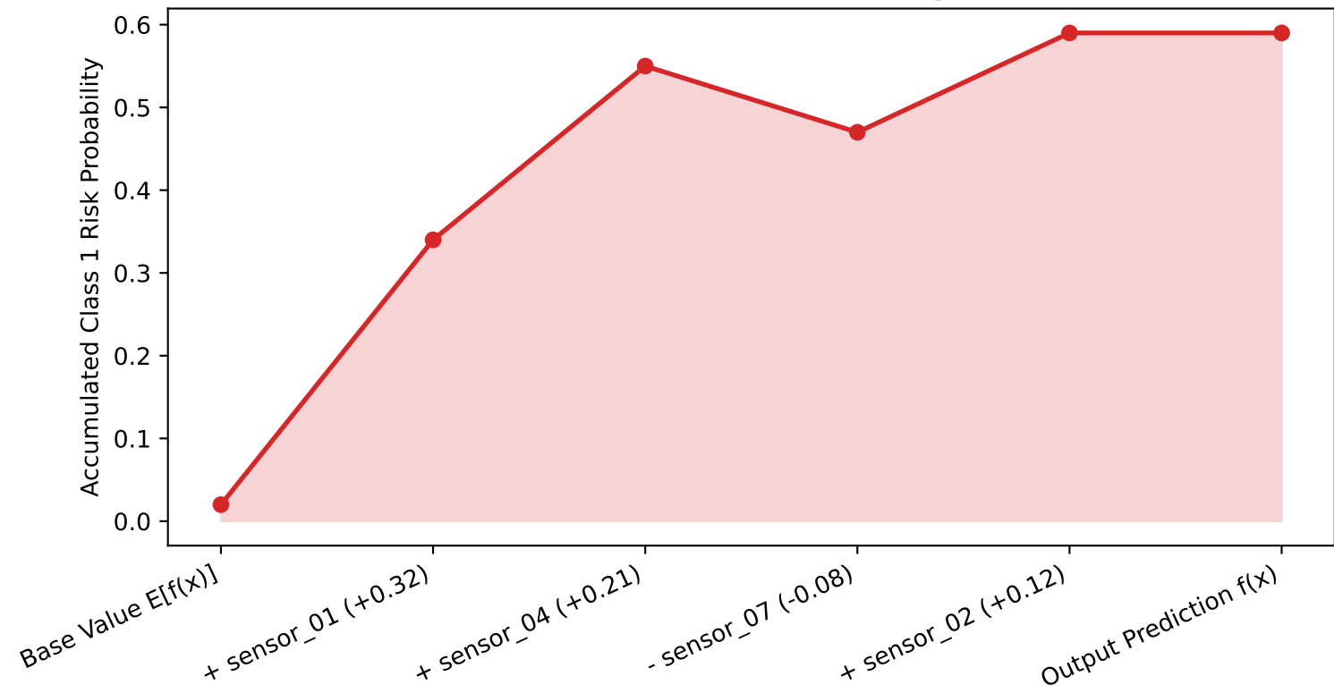
SHAP Waterfall Instance Attributions (Sample #42 Breakdown)
