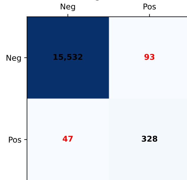
LightGBM
