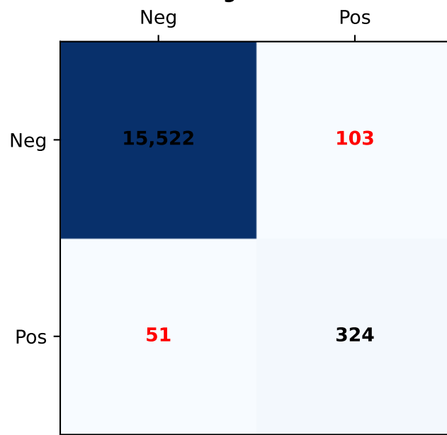
Voting Ensemble
