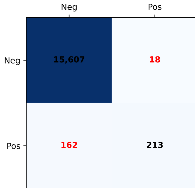
Voting Ensemble
