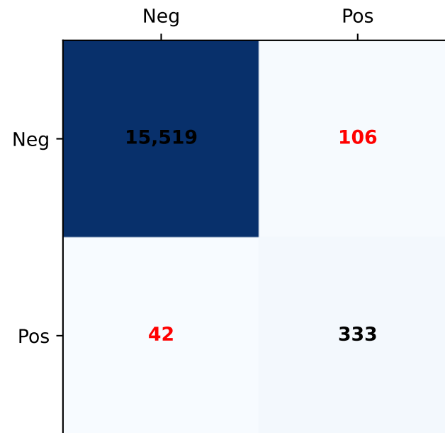
Proposed Asymmetric Ensemble (Ours)
