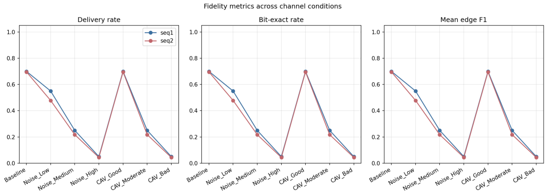
Figure 6.8: The superseded figure, retained as evidence. Three panels plot the identical curve, and the rise at CAV_Good is not a recovery but Baseline replotted under a duplicate configuration.
