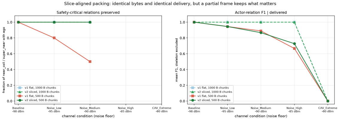
Figure 6.6: Format v1 against v2. The 1000 B pair coincide because only 2 of 20 frames span more than one chunk at that size. The 500 B pair separate: v1 falls to 0.80 then 0.50; v2 holds 1.00.
