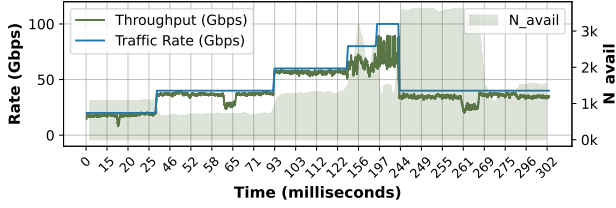
Figure 6. Toasty buffer adjustment with different traffic rates
