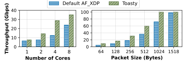
Figure 13. Toasty with varying packet size and CPU cores
