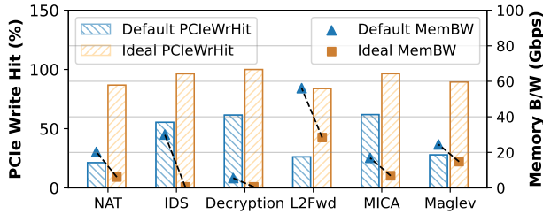
Figure 3. PCIe write hit rate and memory bandwidth usage
