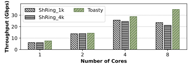
Figure 15. Toasty vs. ShRing
