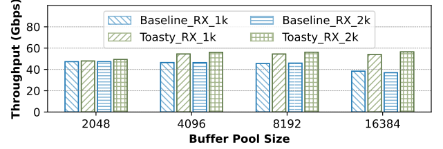
Figure 8. Toasty vs. baseline AF_XDP with varying UMEM
