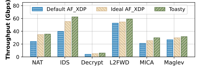
Figure 11. No-drop rate: Toasty vs. baselines
