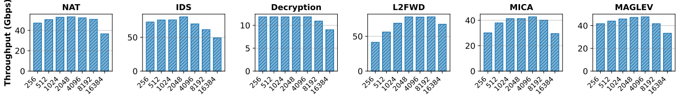
Figure 2. Application throughput vs. size of the packet buffer pool
