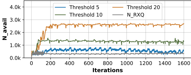
Figure 19. Number of available buffers vs. k
