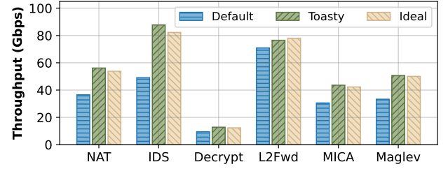
Figure 7. Single core throughput: Toasty vs. baselines
