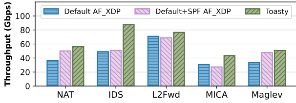
Figure 16. Toasty vs. software prefetching
