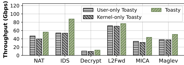
Figure 18. User-space only and kernel-space only variants
