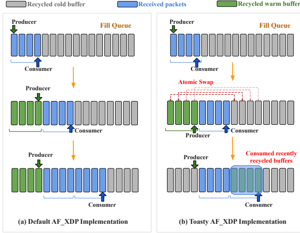
Figure 5. Toasty userspace changes in AF_XDP
