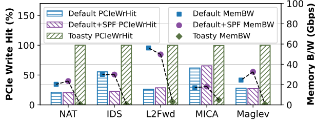
Figure 17. PCIe write hit rate and memory BW with SPF
