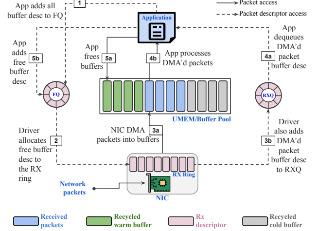
Figure 1. Lifecycle of a packet buffer
