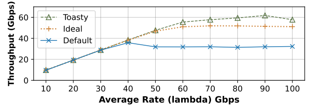
Figure 10. Throughput with Poisson traffic
