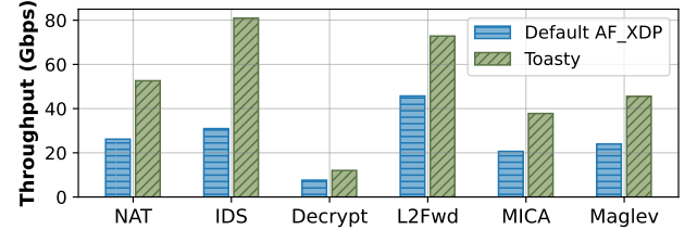
Figure 12. Toasty vs. baseline with co-located workloads
