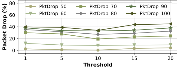
Figure 20. Performance of Toasty for different values of k
