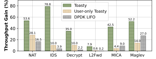
Figure 14. Toasty vs. User Toasty vs. DPDK LIFO mempool
