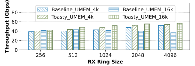
Figure 9. Toasty vs. baseline AF_XDP with varying RX ring
