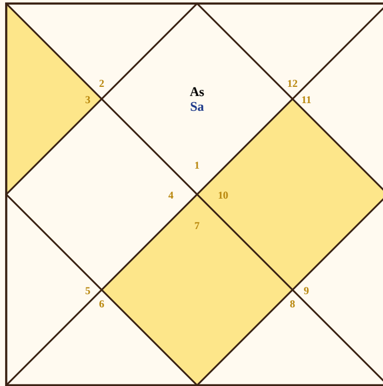
Figure 6.3: Saturn in the 1st supervises the 3rd (effort), the 7th (partnerships) and the 10th (career).
