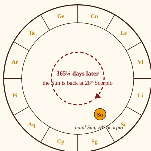
Figure 15.3: Once a year the Sun arrives back at its natal degree (here 28° Scorpio, Chart A's Sun). The moment of that return is the birth of the annual chart. It falls within about a day of the calendar birthday and at a different clock time every year.
