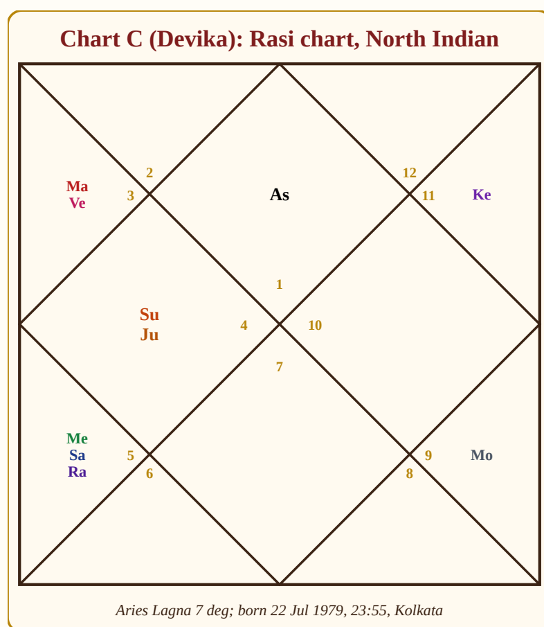
Figure 25.9: Chart C, North Indian style. Sun and Jupiter in the 4th (Cancer); Mars and Venus in the 3rd (Gemini); Mercury, Saturn and Rahu in the 5th (Leo); Moon in the 9th (Sagittarius); Ketu in the 11th (Aquarius).
