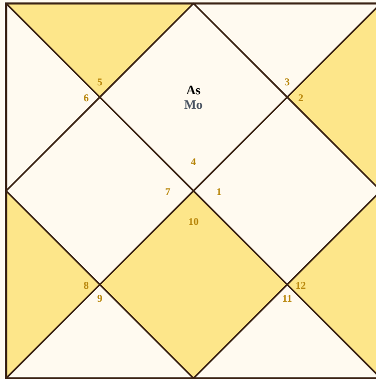
Figure 14.2: The same frame for Jupiter: 2, 5, 7, 9 and 11 from the Moon. From each of these positions, Jupiter's trinal aspects land on other houses in the same list.
