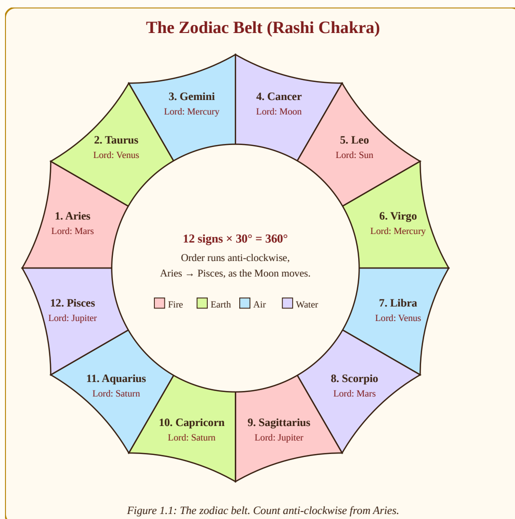
Figure 1.1: The zodiac belt. Twelve signs of 30^\circ each make the full 360^\circ circle. The order runs anti-clockwise — the same direction the Moon and planets move against the stars.
