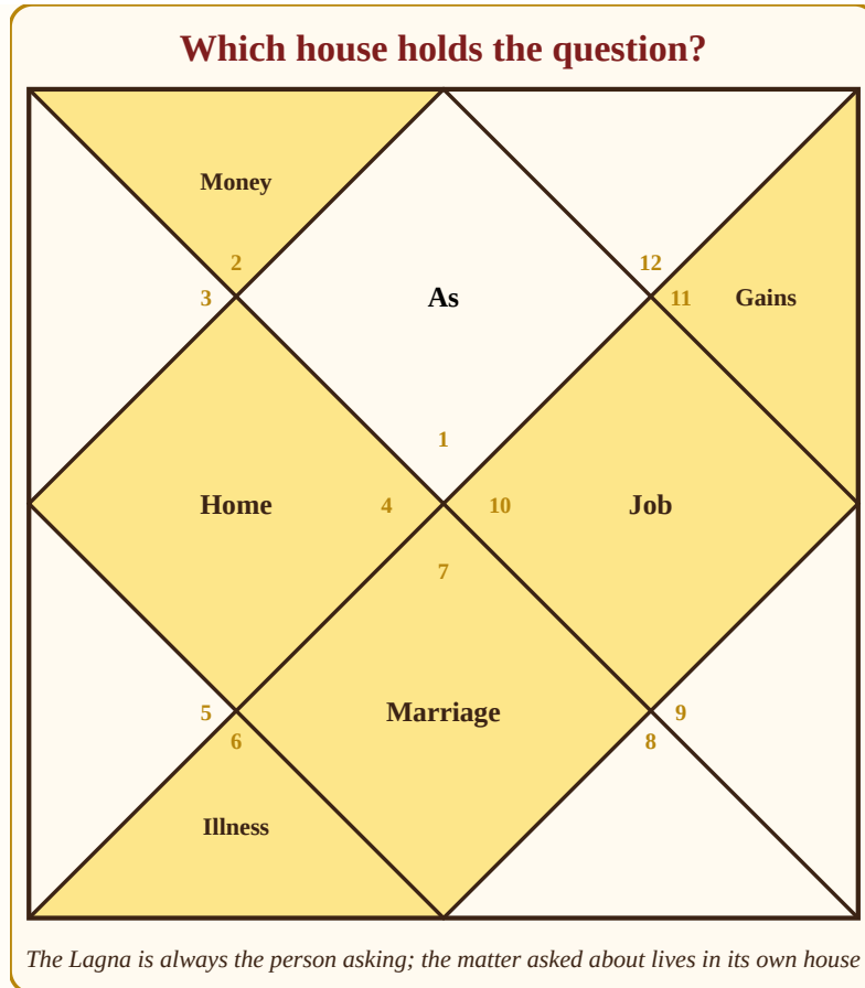
Figure 17.2: The querent is always the 1st house. Money lives in the 2nd (and gains in the 11th), home and lost household objects in the 4th, illness and enemies in the 6th, marriage and the "other party" in the 7th, job and career in the 10th.
