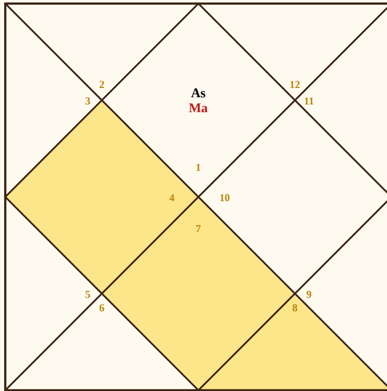
Figure 6.1: Mars in the 1st. The shaded houses receive its full gaze: the 4th (leap forward), the 7th (face to face), and the 8th (strike behind).
