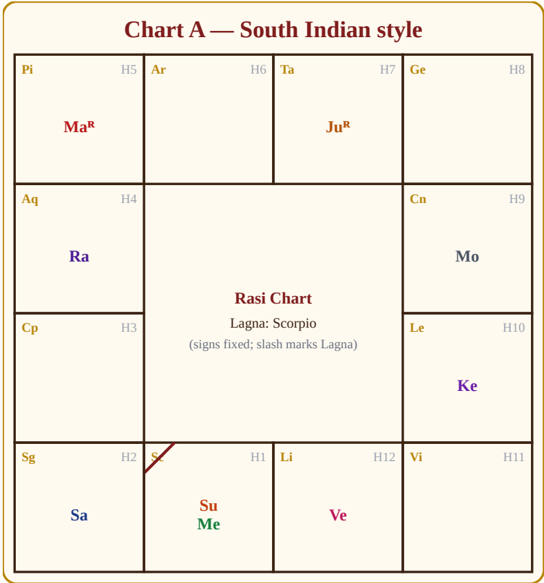
Figure 1.4: The same chart in the South Indian format. Pisces is always top-left; the signs run clockwise; the slash marks the Lagna in Scorpio.
