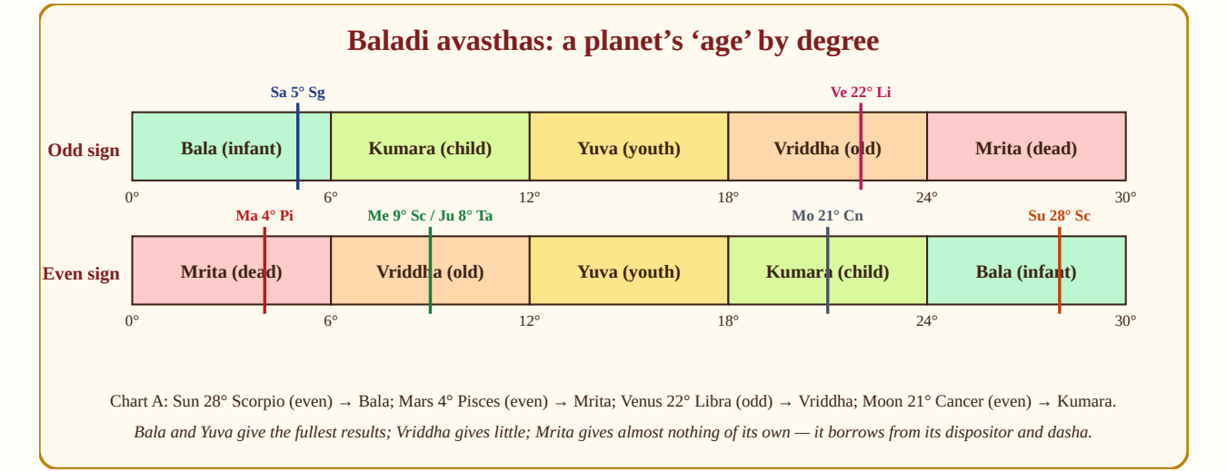
Figure 12.4: The five age bands. Odd signs read left to right, even signs right to left. Meera's planets are marked: the Sun at 28° of even Scorpio is an infant; Mars at 4° of even Pisces is "dead".
