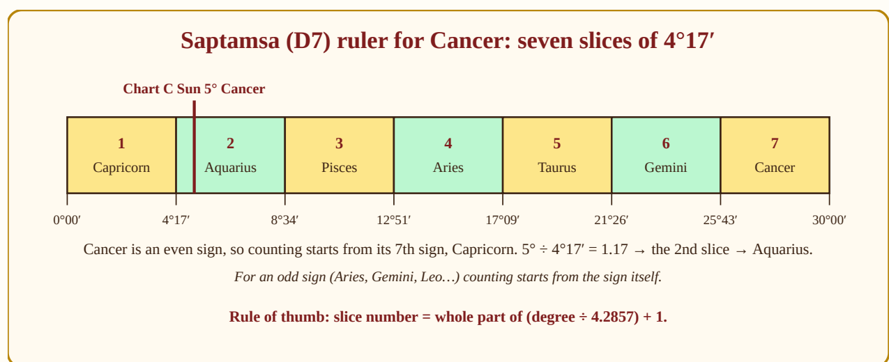
Figure 21.2: The D7 ruler for Cancer. Seven slices of 4^{\circ}17' , counted from the 7th sign because Cancer is even. The Sun at 5^{\circ} lands in the second slice, Aquarius.
