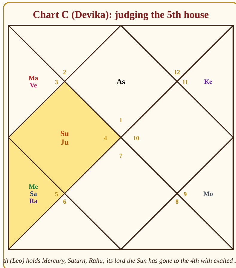
Figure 9.2: Chart C. The 5th house Leo holds Mercury, Saturn and Rahu. Its lord, the Sun, has gone to the 4th house Cancer, where exalted Jupiter also sits.
