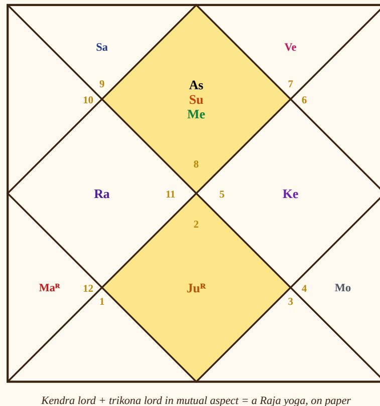
Figure 10.1: Chart A. The 10th lord Sun in the 1st and the 5th lord Jupiter in the 7th look straight at each other — a Raja yoga by mutual aspect.
