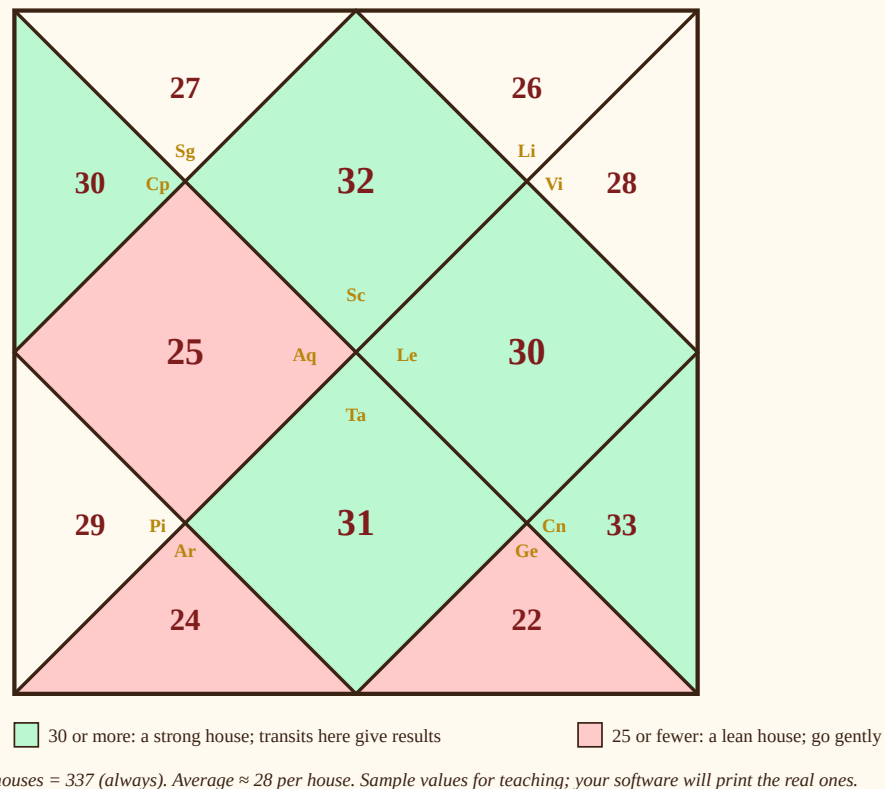
Figure 12.3: A sample Sarvashtakavarga laid on Chart A's houses (Scorpio Lagna). Green houses have 30 or more bindus, red houses 25 or fewer. The twelve numbers always total 337. Values invented for teaching; your software prints the real ones.
