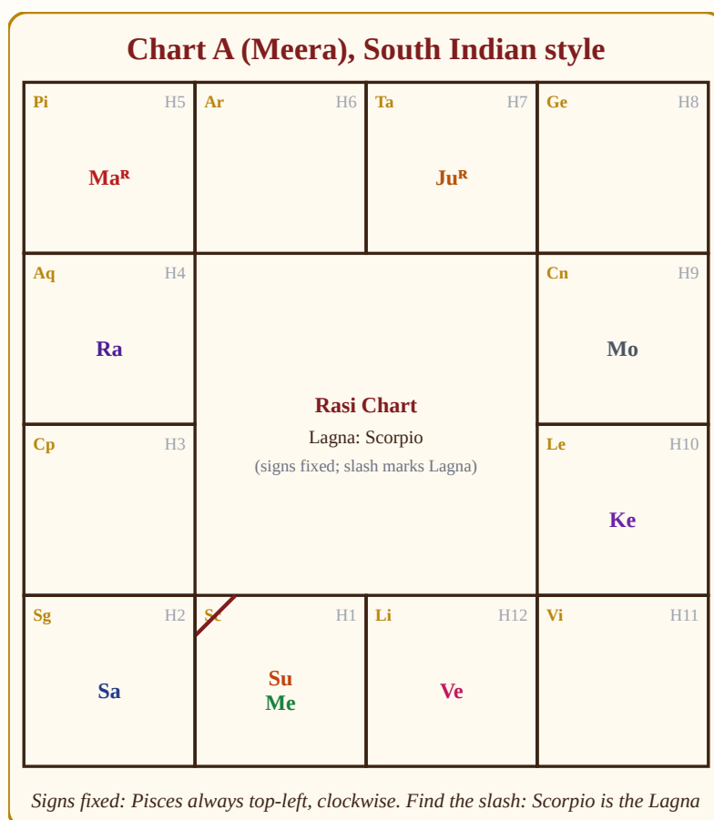
Figure 5.2: The same chart, South Indian style. Signs fixed and running clockwise from Pisces at top-left. The slash in the Scorpio box marks the Lagna. Count clockwise from there for houses 2 to 12.
