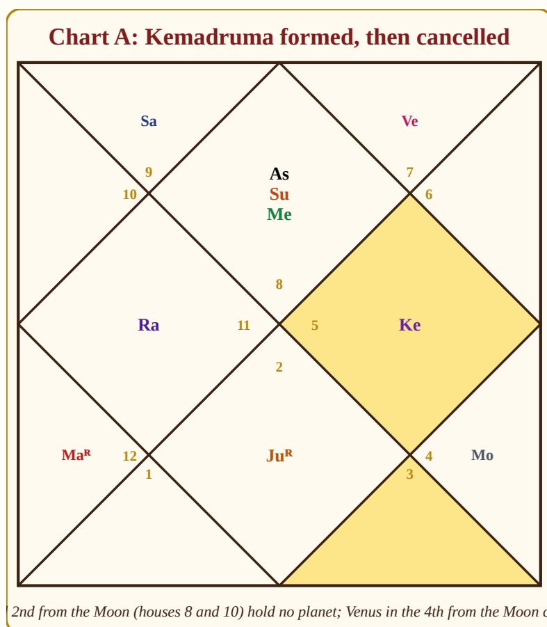
Figure 10.5: Chart A. The 12th and 2nd from the Moon (houses 8 and 10) hold no counting planet, so Kemadruma forms; Venus in the 4th from the Moon and several planets in kendras from the Lagna cancel it.
