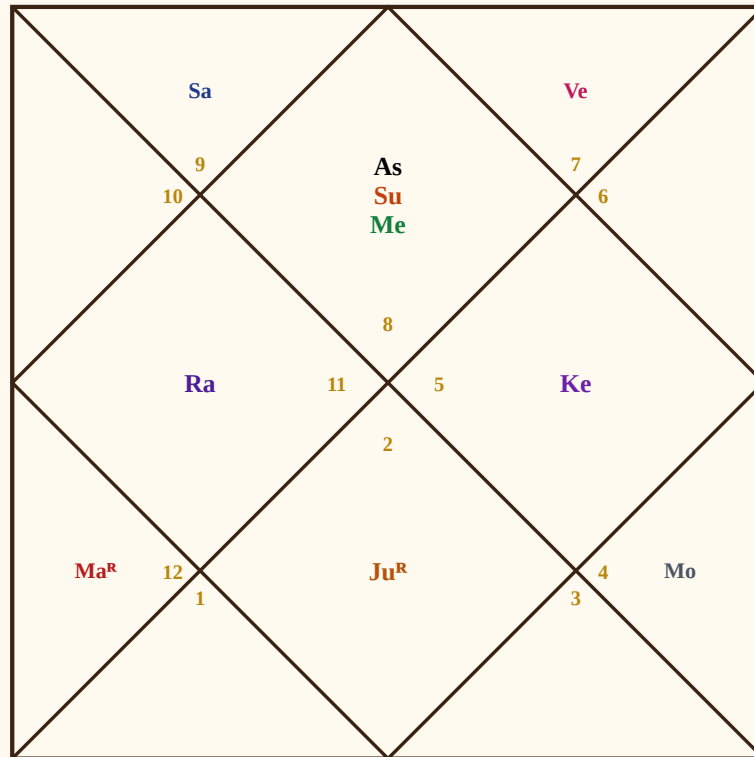
Figure 3.4: Chart A. Sun at 28° Scorpio, Mercury at 9° Scorpio — same sign, 19° apart. Mercury is well outside its 14° orb, so it is not combust, and the Budha–Aditya yoga holds.
