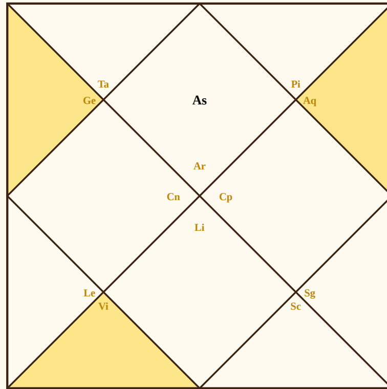
Figure 8.1: Aries Lagna. The shaded houses (3rd Gemini, 6th Virgo, 11th Aquarius) are the ones whose lords turn malefic. Read off the owner of each shaded sign: Mercury, Mercury, Saturn.
