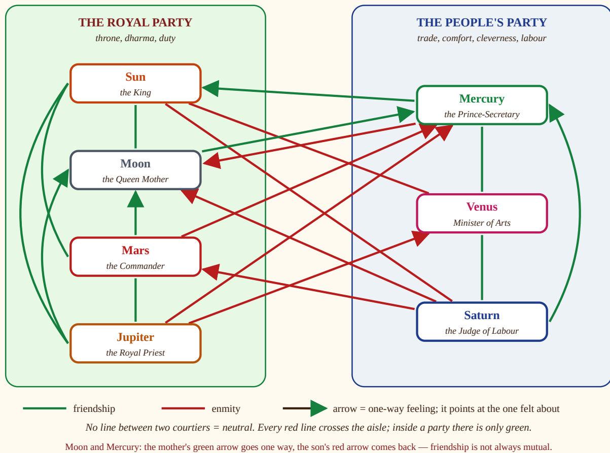
Figure 3.3: The two parties. Green lines are friendships, red lines enmities; an arrowhead means the feeling runs one way only; pairs with no line are neutral to each other.
