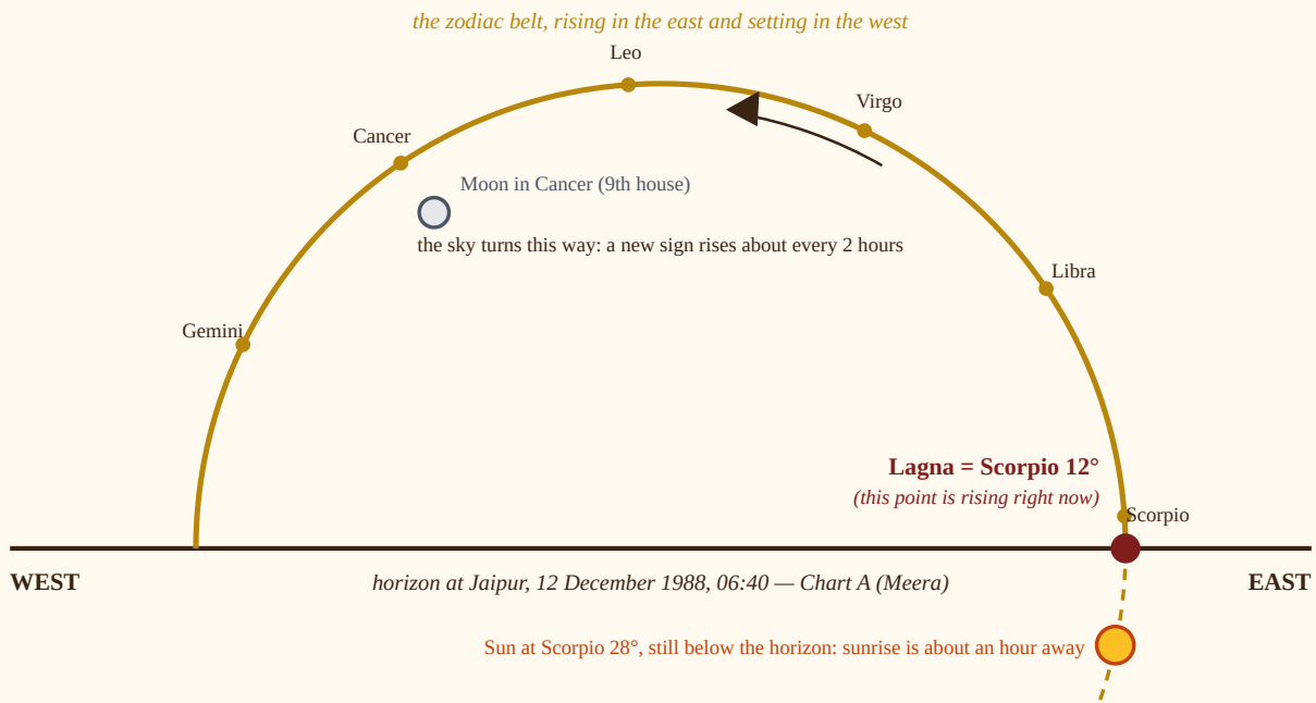
Figure 5.5: The Lagna is simply the point of the zodiac on the eastern horizon. Meera was born a little before sunrise, so her Lagna is in the Sun's sign, a few degrees behind the Sun.
