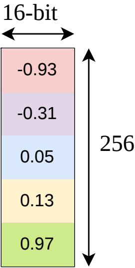
Dictionary
