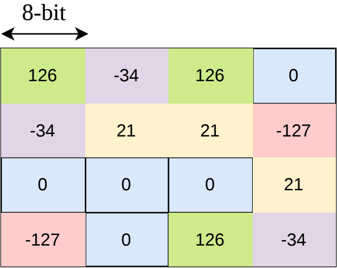
Weight indices
