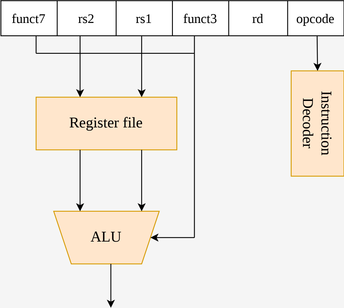
R-type instruction
