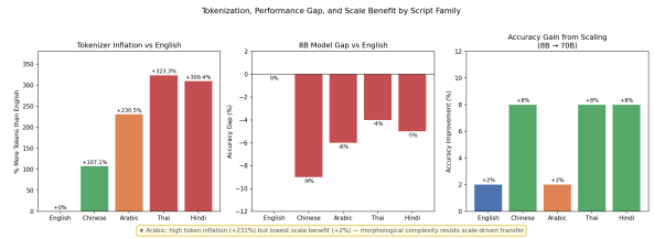
Figure 2: Left: Tokenizer inflation vs English by language. Centre: 8B model accuracy gap vs English. Right: Accuracy gain from scaling (8B to 70B). Arabic shows moderate token inflation (+231%) but the lowest scale benefit (+2%), suggesting morphological complexity as the key factor.
