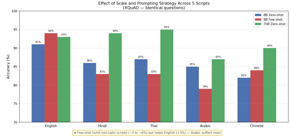
Figure 1: Accuracy across five languages under three conditions: 8B zero-shot, 8B few-shot, and 70B zero-shot. Few-shot hurts all non-Latin scripts except Chinese; scaling helps all languages but Arabic benefits least.
