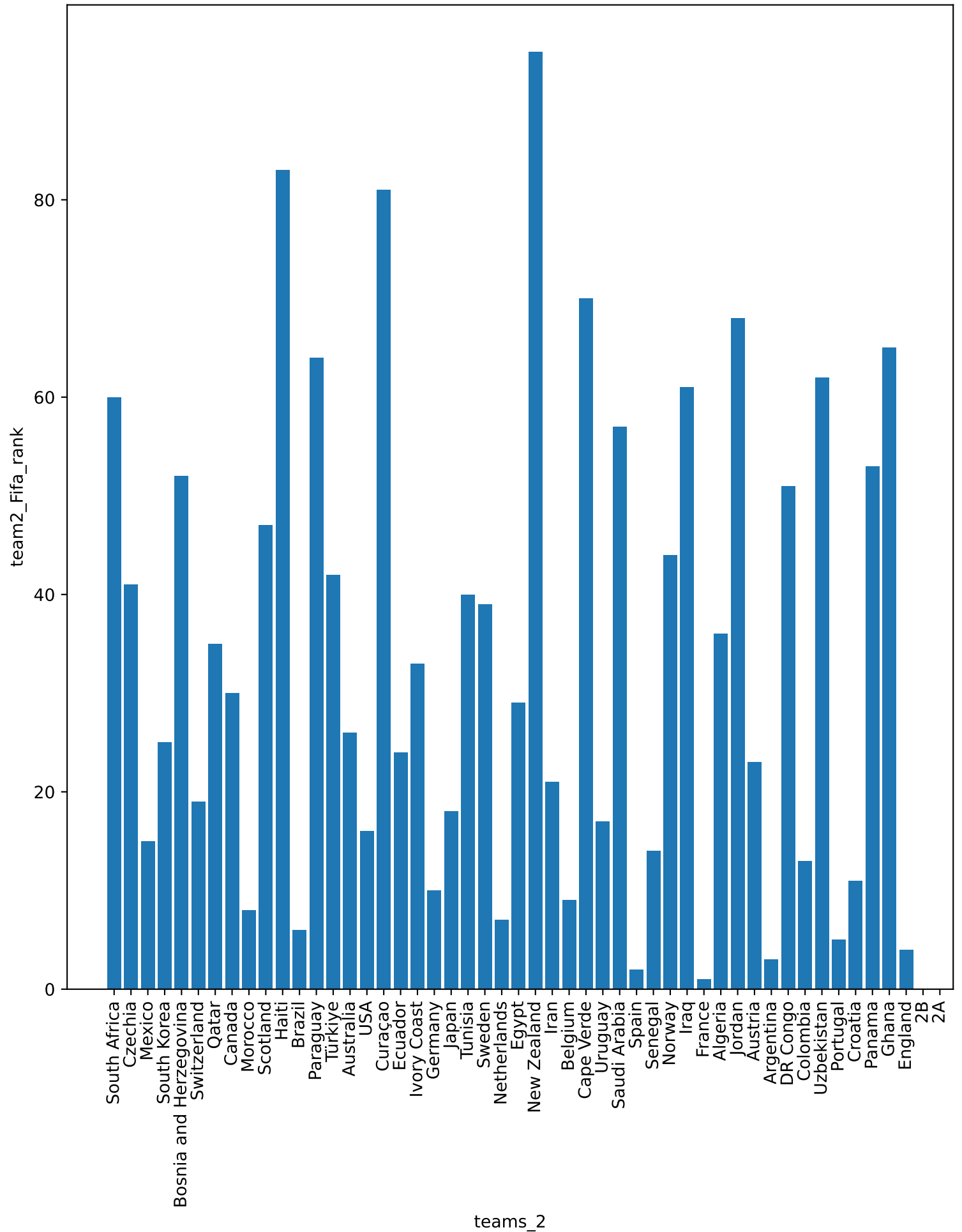
Rank analysis
