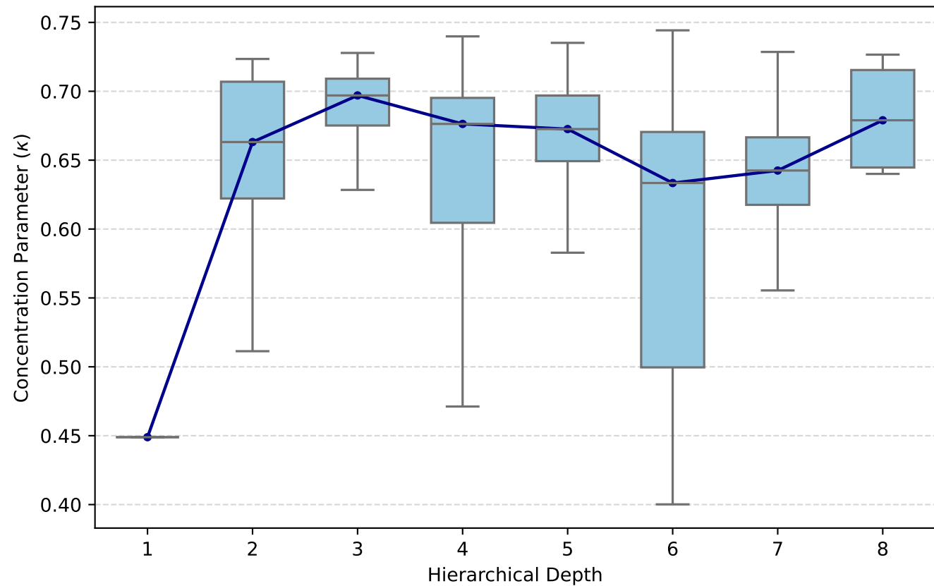
Semantic Certainty vs. Depth: science (Median Trend Correlation: 0.48)
