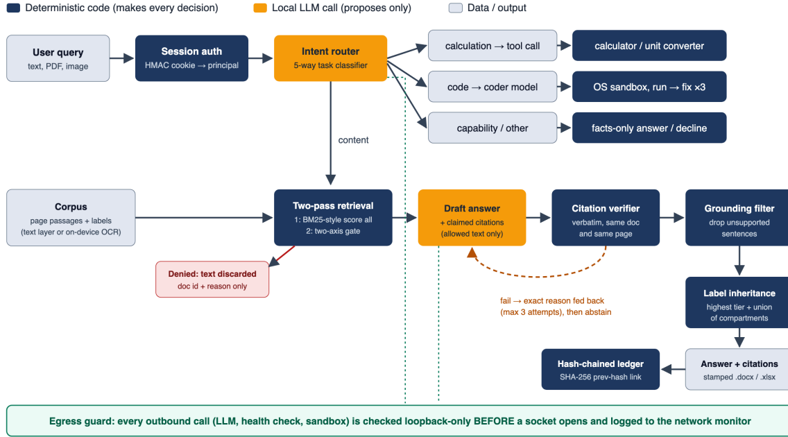
Fig. 1. Sovereign_AI request path. The router sends each question to one of five paths; the document path passes through a two-axis gate, drafting, verbatim citation verification and a grounding filter, with retry and abstention. All outbound calls pass a loopback-only egress guard.
