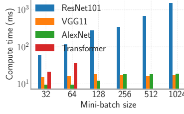
(b) SSP compute time
