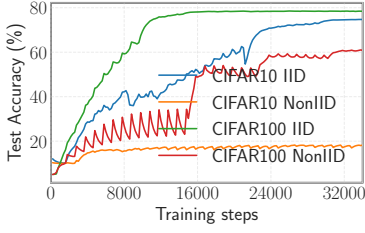
(a) FedAvg IID vs. non-IID data
