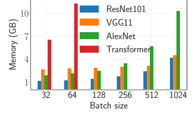
(c) SSP memory consumption
