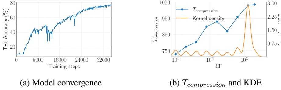
Figure 5.8: ResNet101 deployed with GraVAC on geometric scaling policy. We evaluate more candidate CFs under this policy as seen from the iteration density distributions.
