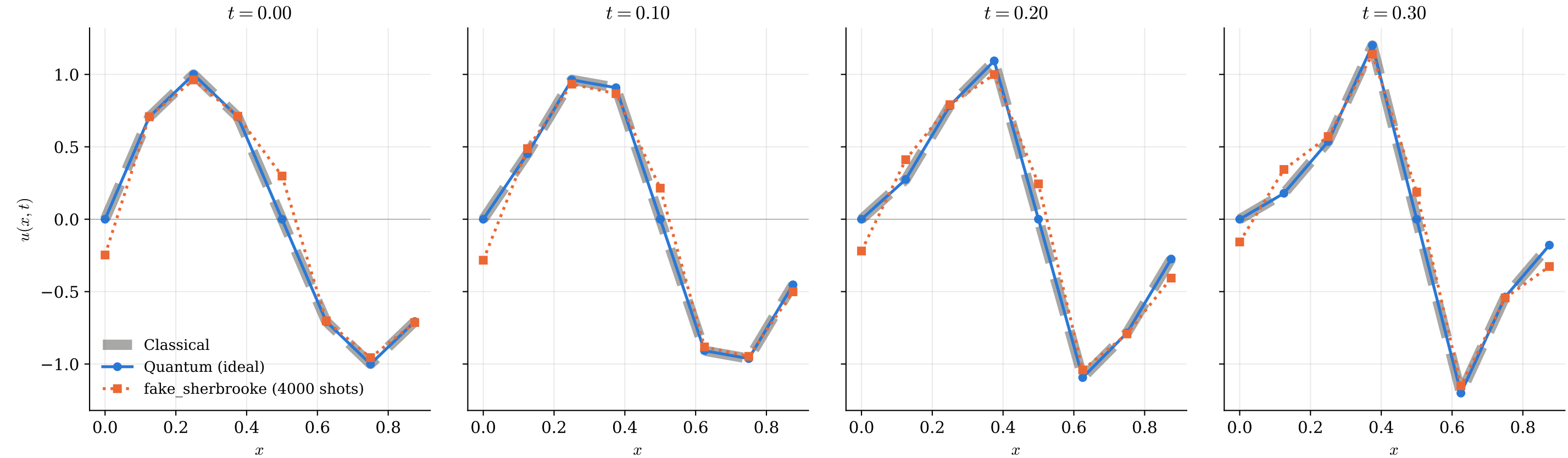
Variational Burgers time-propagation ( \nu = 0.01 , dt = 0.1 )
