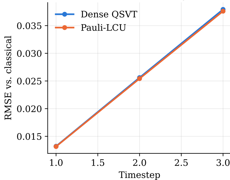
Solution accuracy
