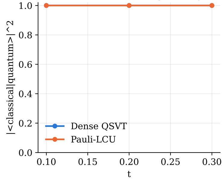
Amplitude-encoding fidelity
