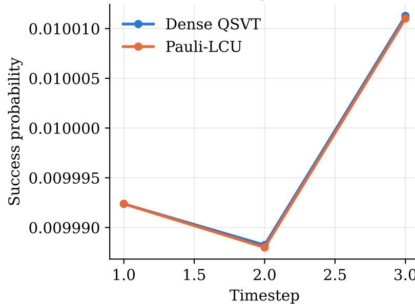
Block-encoding post-selection
