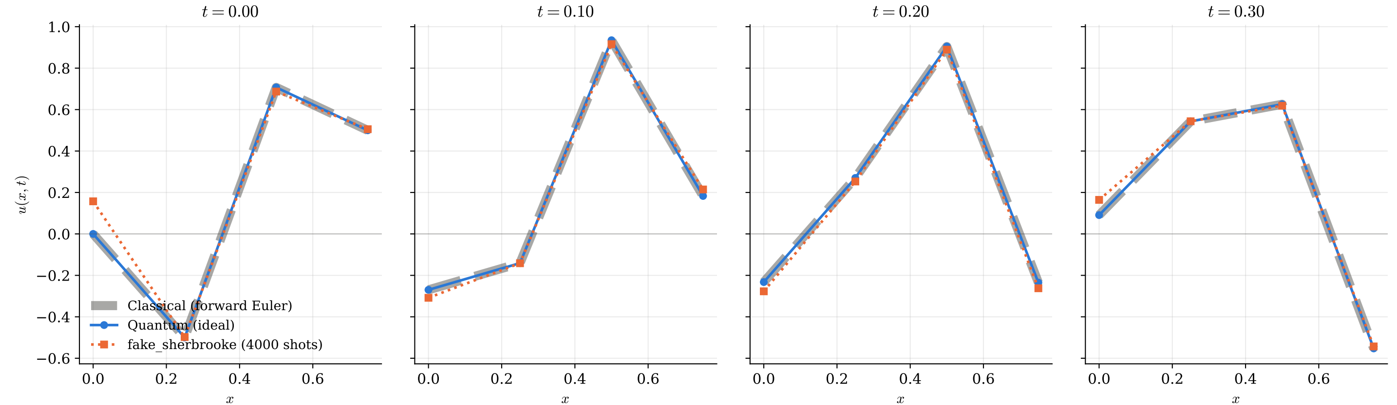
KdV time-propagation via natural-gradient descent ( \delta = 0.0625 , dt = 0.1 )
