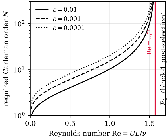
(a) N = \lceil \ln(1/\varepsilon)/\ln(1/R_\star) \rceil
