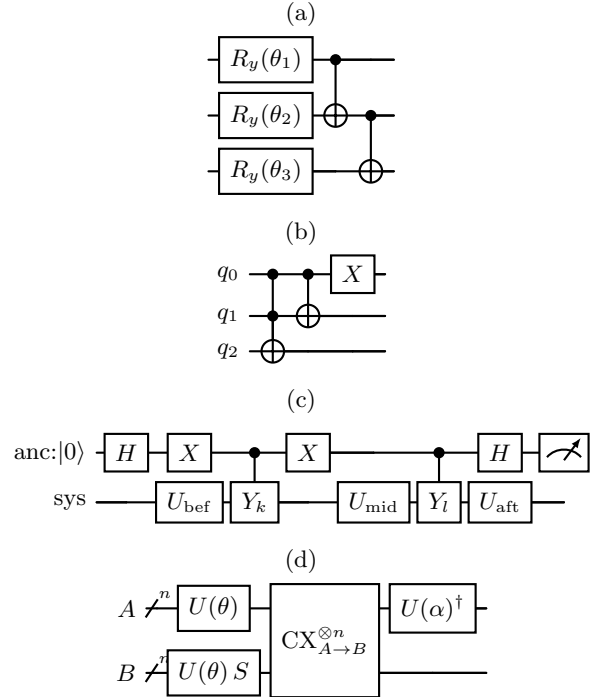
FIG. 4. General circuit primitives: (a) one repetition of the R_y /CNOT ansatz layer, applied n times in total; (b) the ancilla-free cyclic shift gate S ( n = 3 ; the staircase of (n-1-k) -controlled X 's targeting qubit k , k = n-1, \dots, 1 , then X on qubit 0, extends to any n ); (c) the single-ancilla metric off-diagonal circuit, generator insertions Y_k, Y_l between sub-unitaries U_{\text{bef}}, U_{\text{mid}}, U_{\text{aft}} of the ansatz; (d) the two-register nonlinear cross-term circuit, n -qubit registers A, B , no controlled-ansatz gates anywhere.
