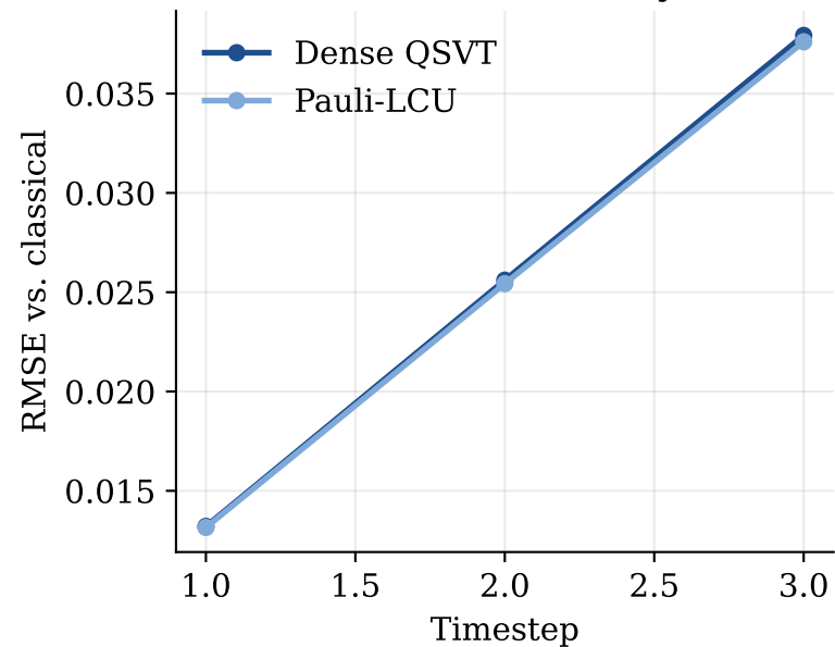
Solution accuracy
