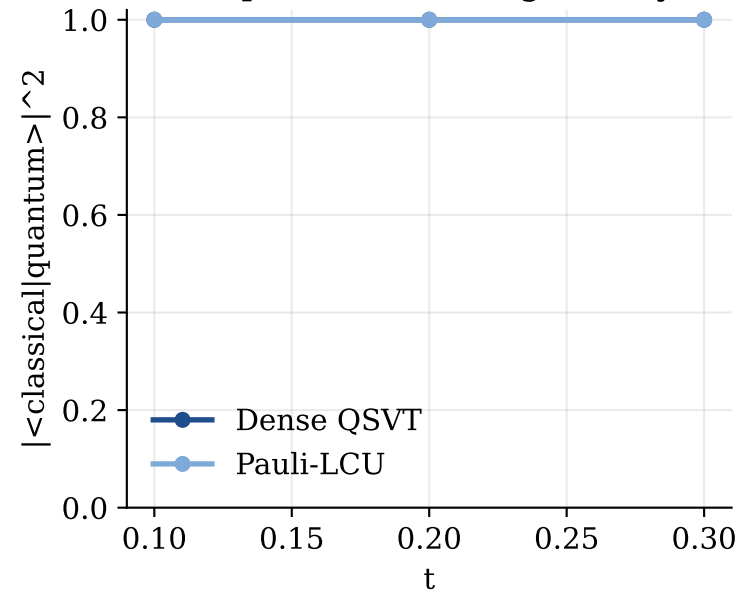
Amplitude-encoding fidelity
