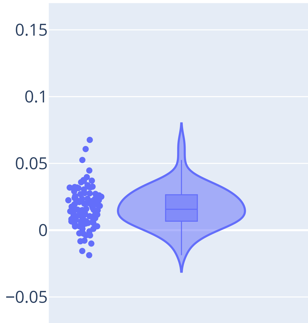
Core + all-MiniLM-L6-v2
