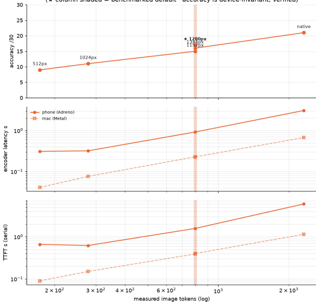
LFM2-VL-450M Q8 — tile quanta: cost jumps at the 1024→1152 px flip (★ column shaded = benchmarked default · accuracy is device-invariant, verified)
