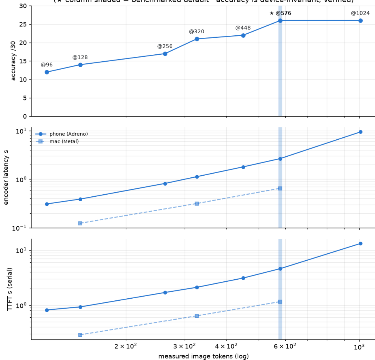
Qwen3-VL-2B Q4_0 — no tiling: one encoder pass, smooth token dial (★ column shaded = benchmarked default · accuracy is device-invariant, verified)
