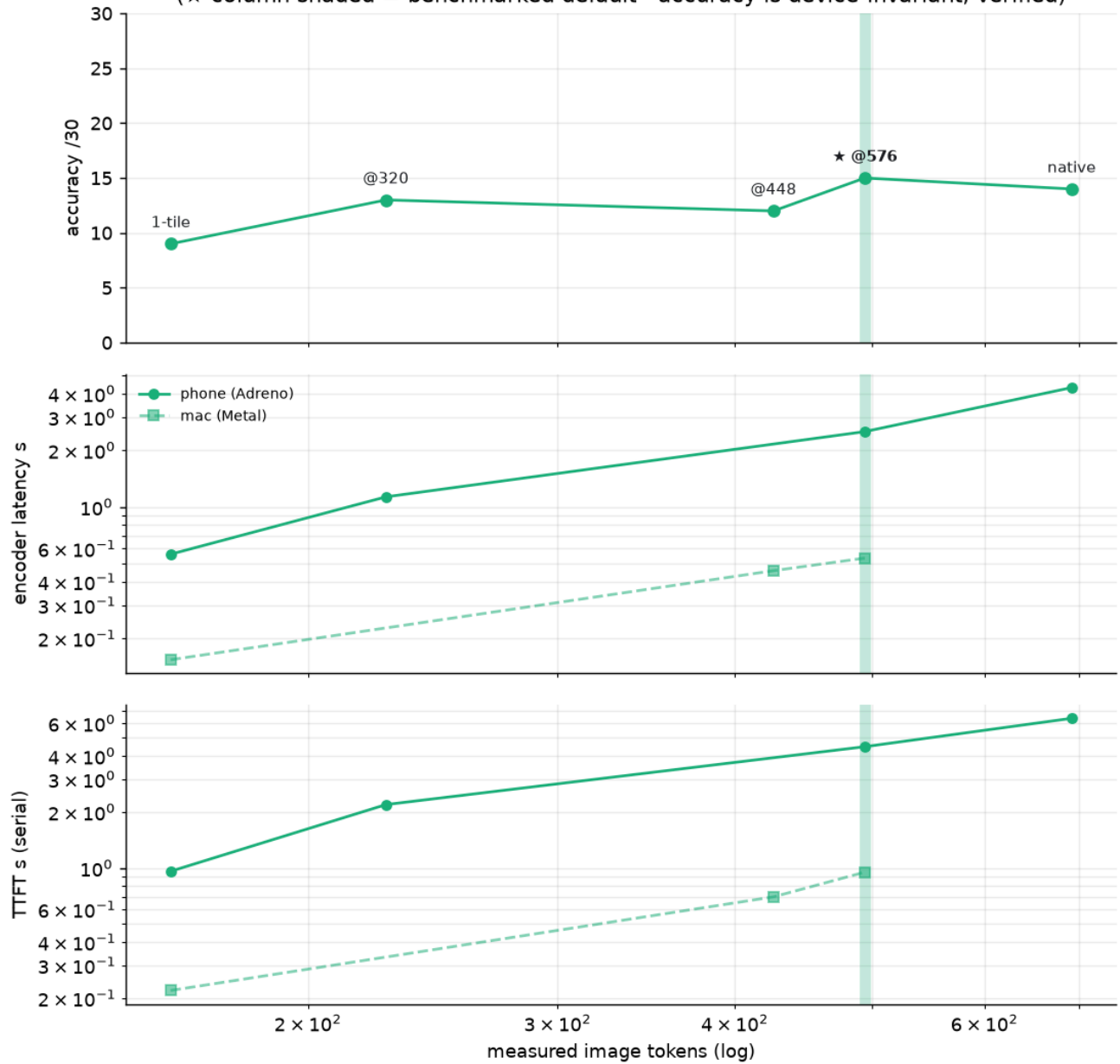
SmolVLM-500M Q8 — capacity-flat: resolution can't buy accuracy (★ column shaded = benchmarked default · accuracy is device-invariant, verified)
