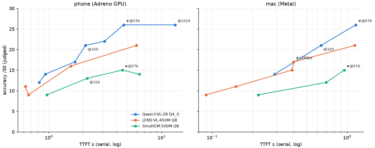
Accuracy vs TTFT — every measured operating point, both devices (★ = benchmarked default)
