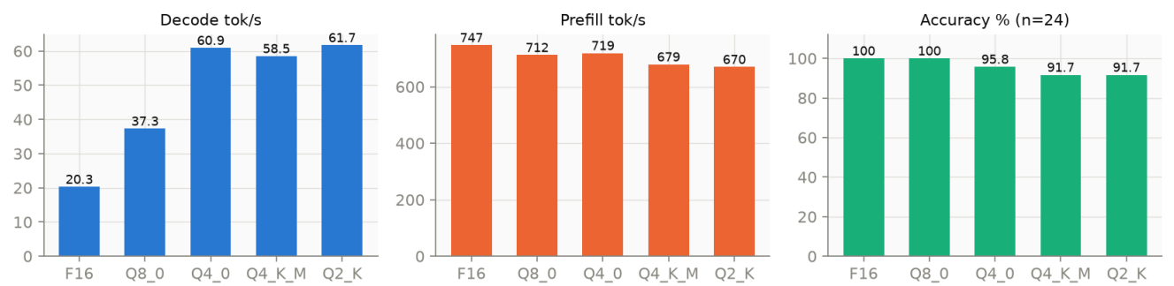
Quantization ladder — Qwen2.5-VL-3B (Mac Metal, cap 576): decode follows bytes, prefill flat, accuracy knee at Q4
