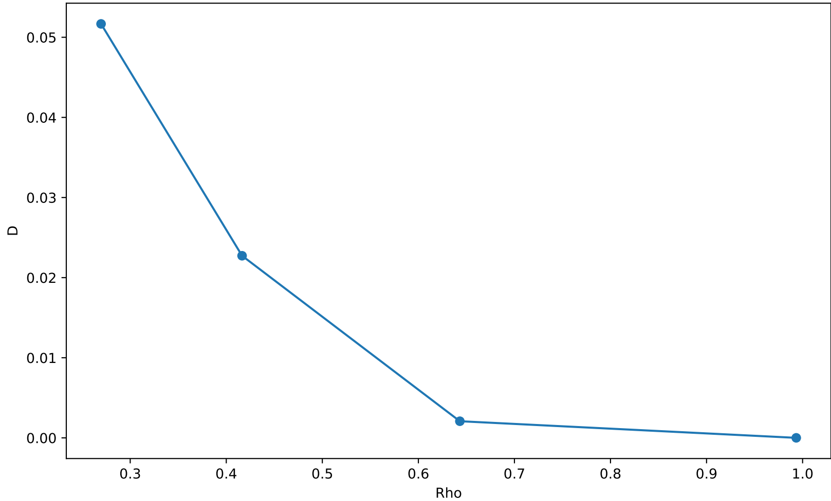
StARS: Rho Selection
