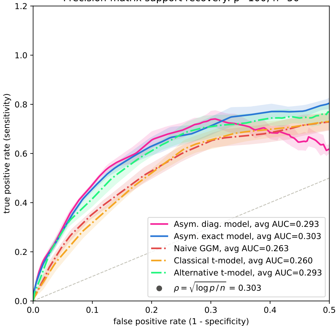
Precision-matrix support recovery: p=100 , n=50
