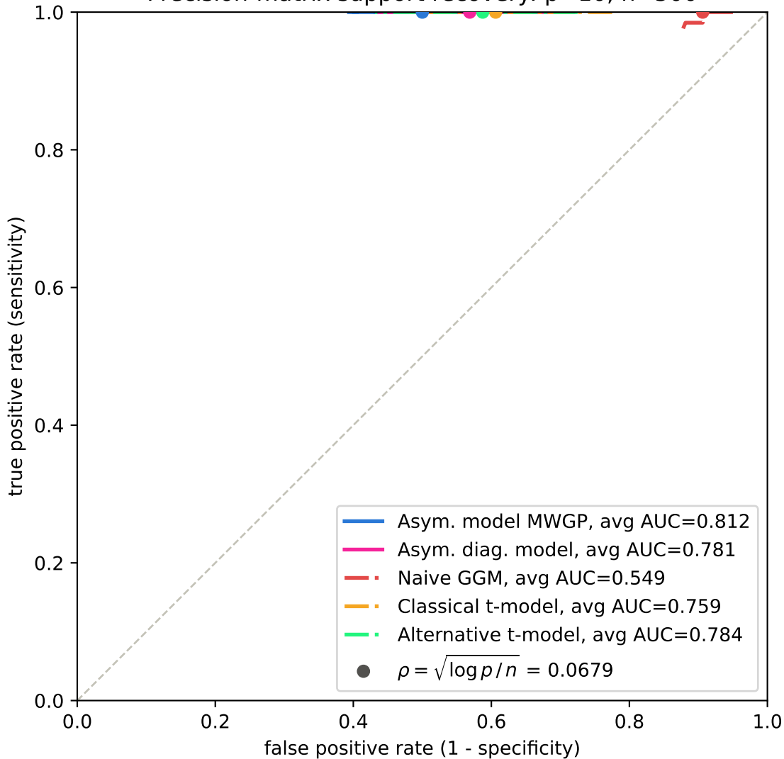
Precision-matrix support recovery: p=10 , n=500
