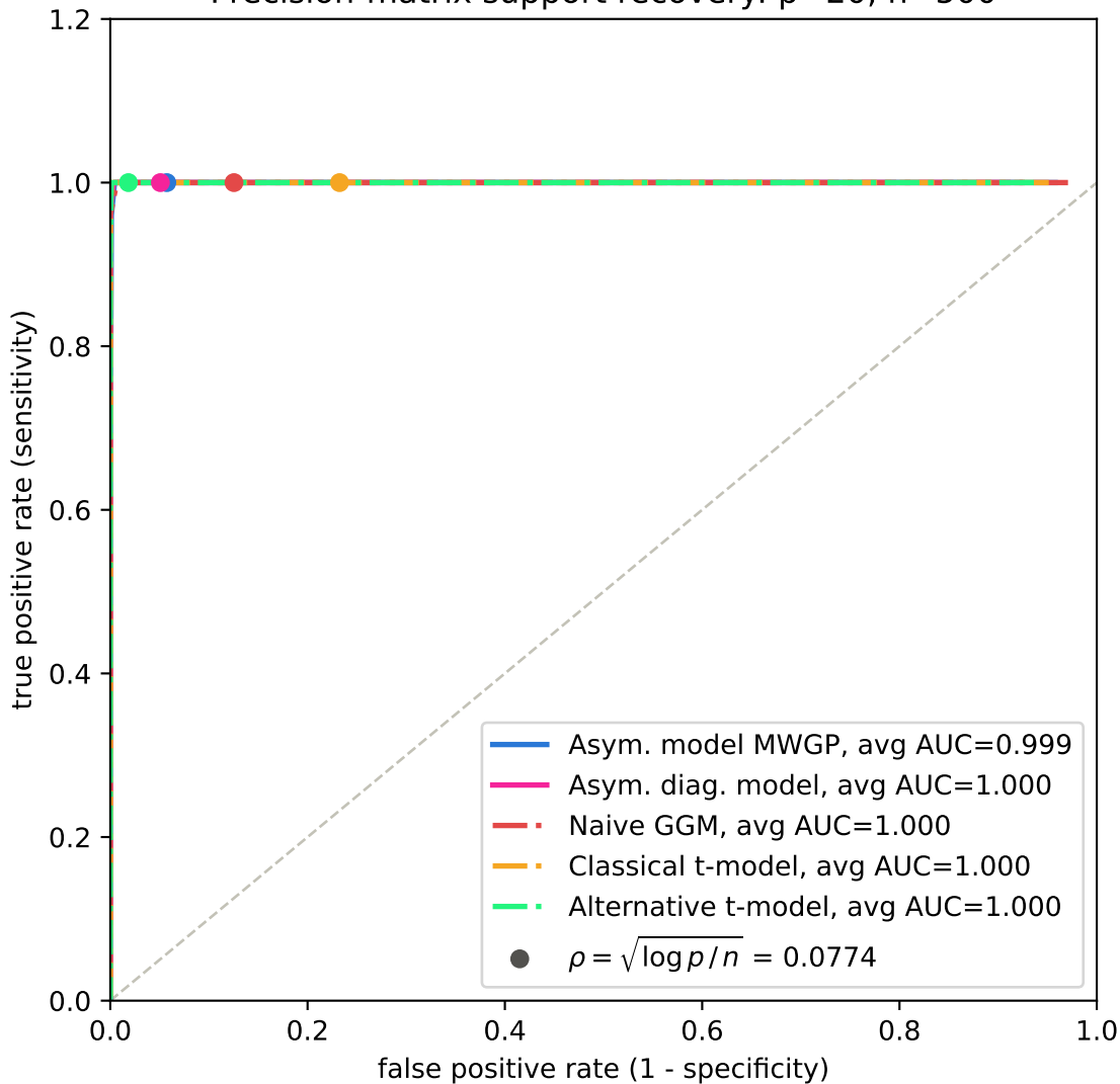
Precision-matrix support recovery: p=20 , n=500
