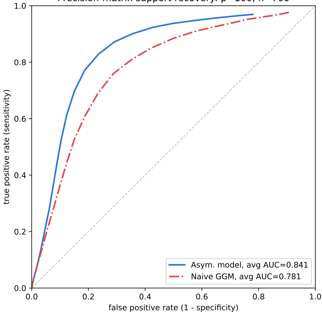
Precision-matrix support recovery: p=100 , n=700
