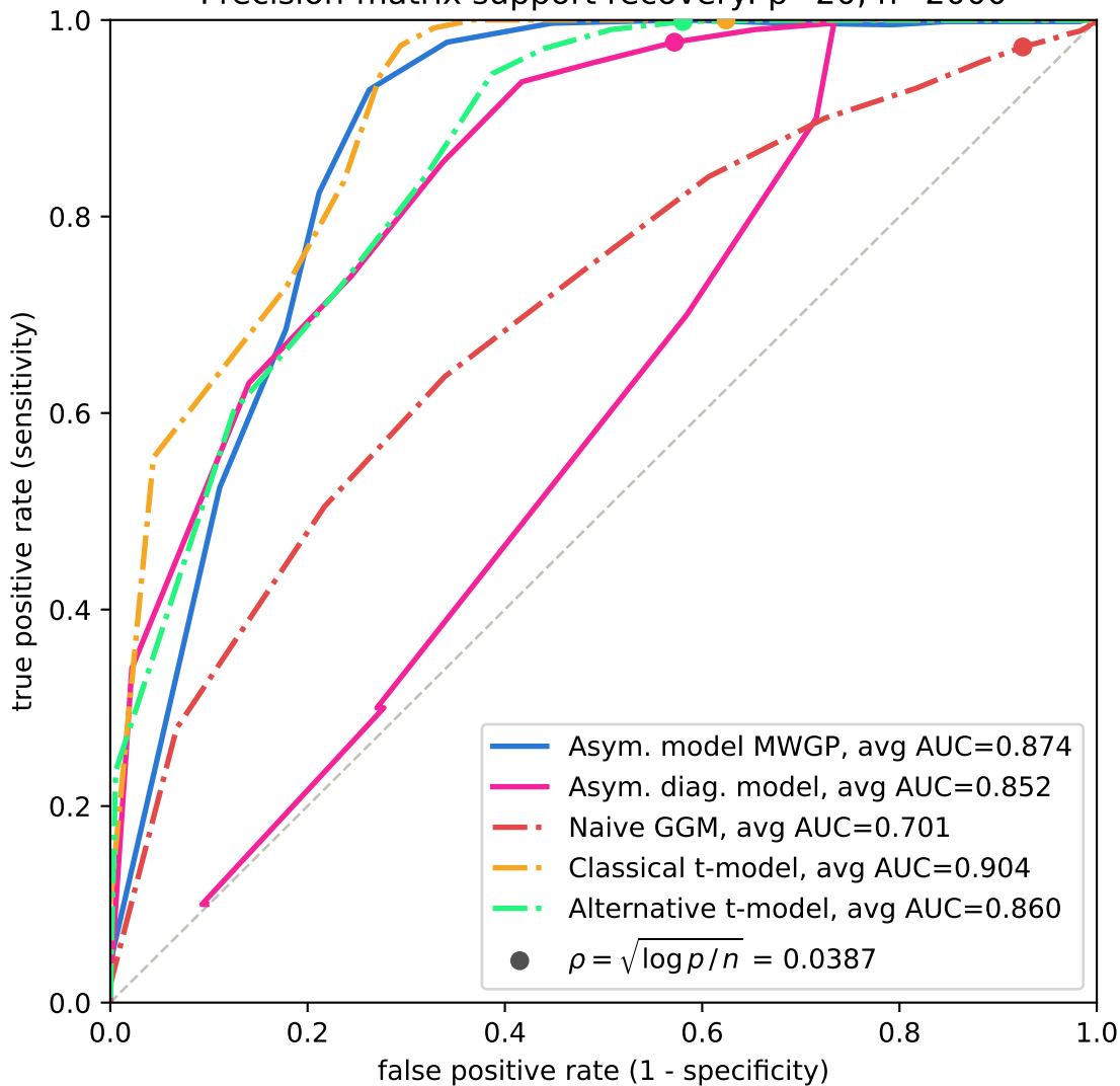
Precision-matrix support recovery: p=20 , n=2000
