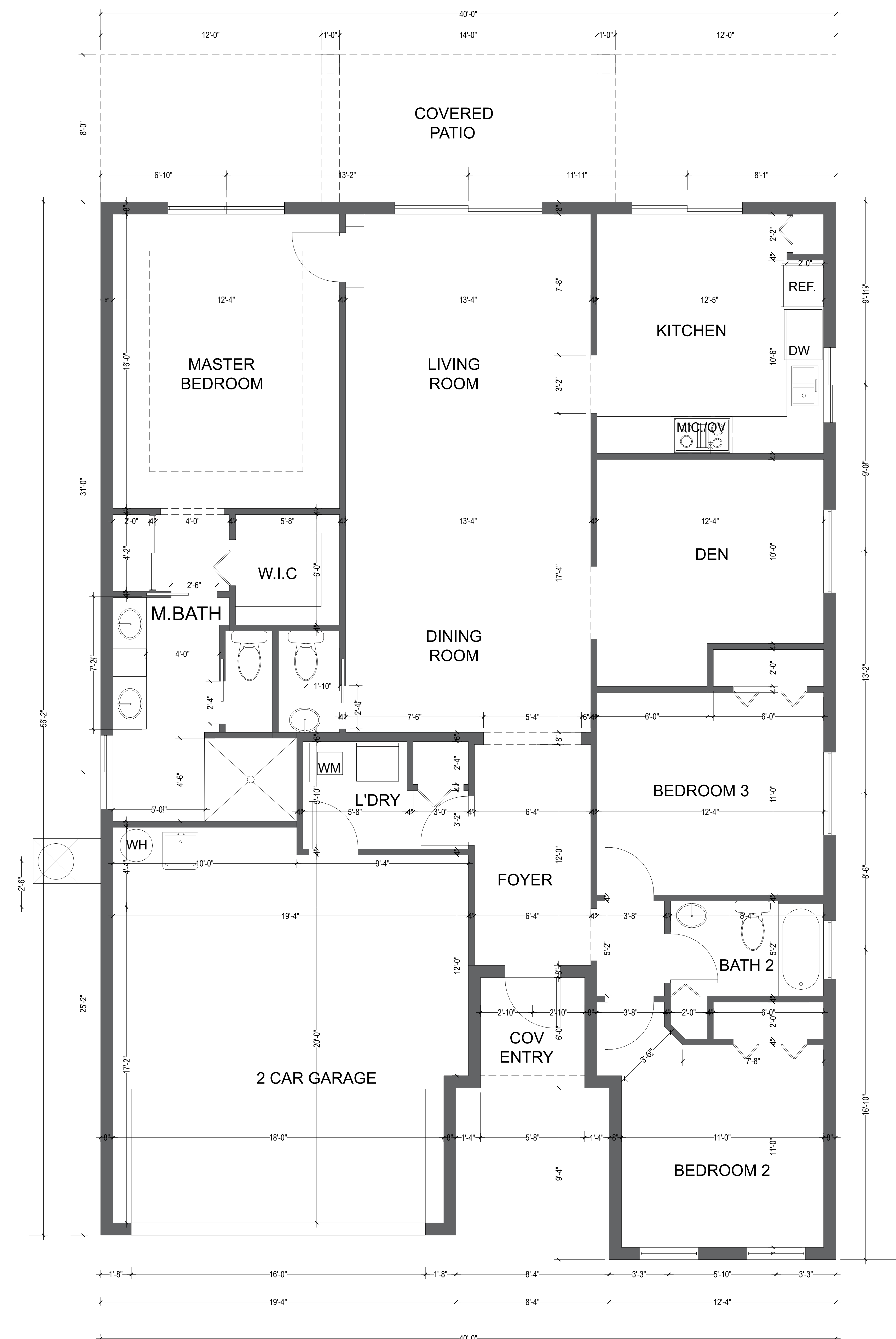
1 0.0 - PROPOSED FLOOR PLAN 3/16" = 1'-0"
