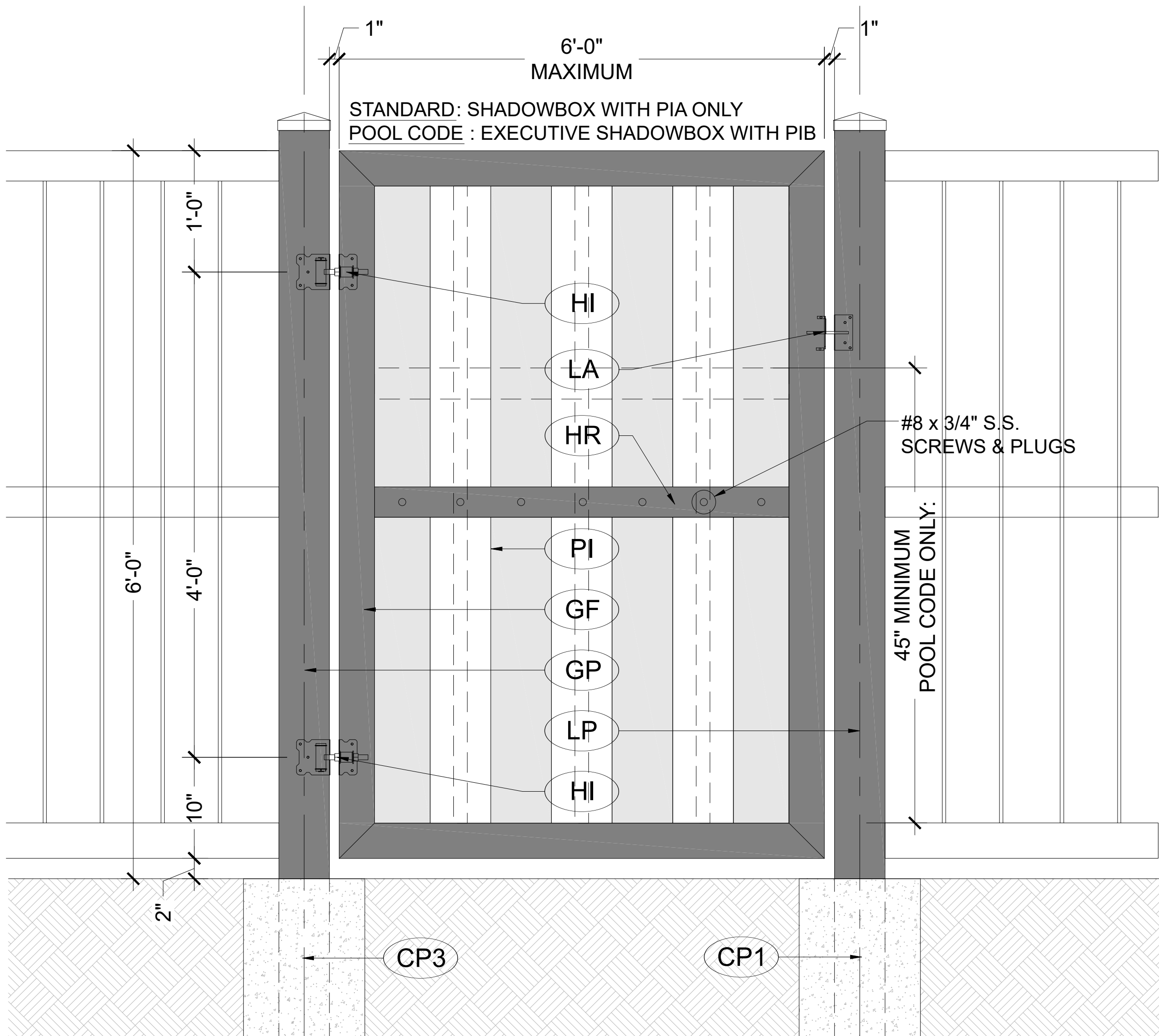
2 SINGLE SWING GATE DETAILS SCALE: 1/2"=1'-0"
