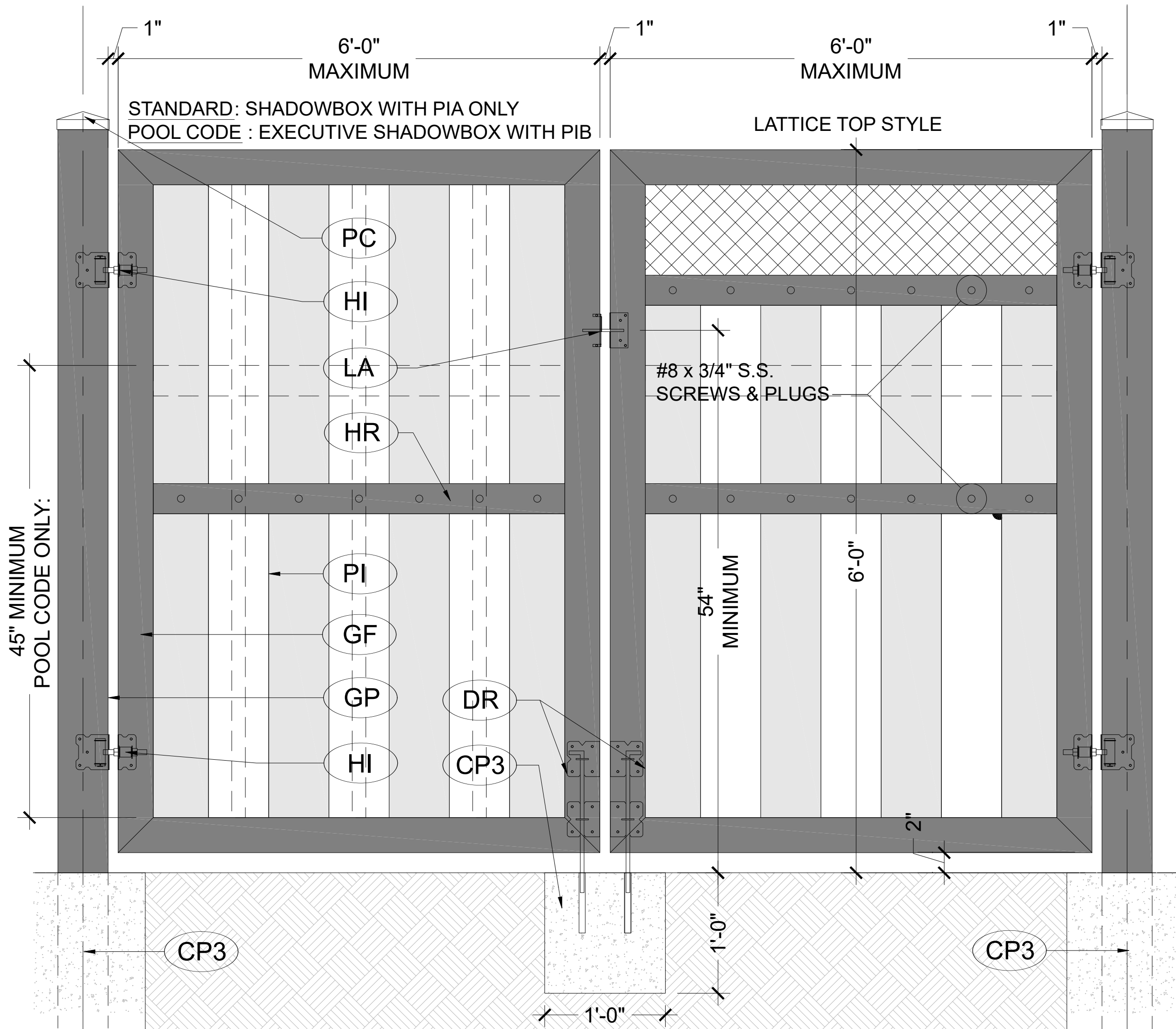
3 DOUBLE SWING GATE DETAILS SCALE: 1/2"=1'-0"
