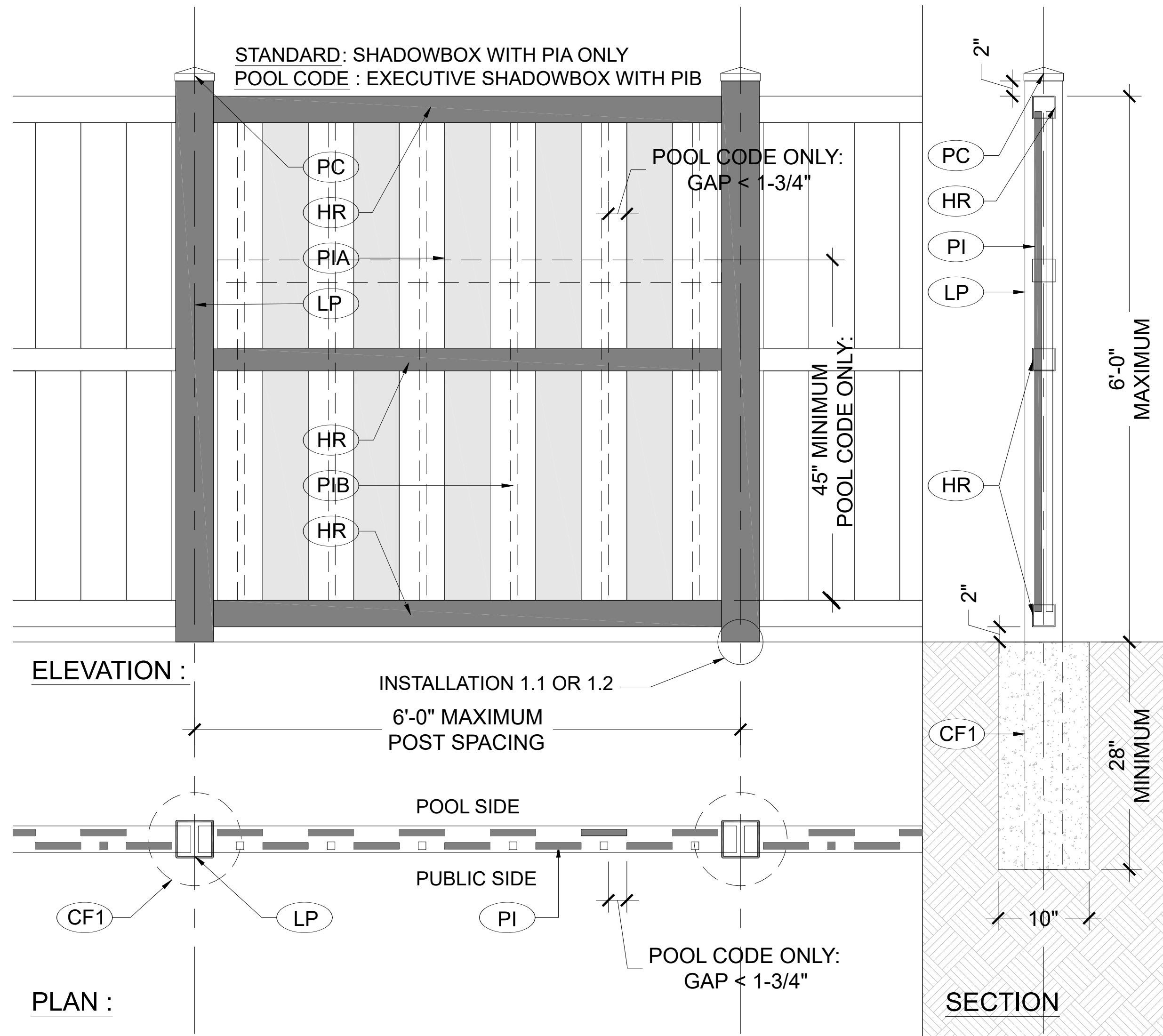
1 FENCING DETAILS SCALE: 3/8"=1'-0"
