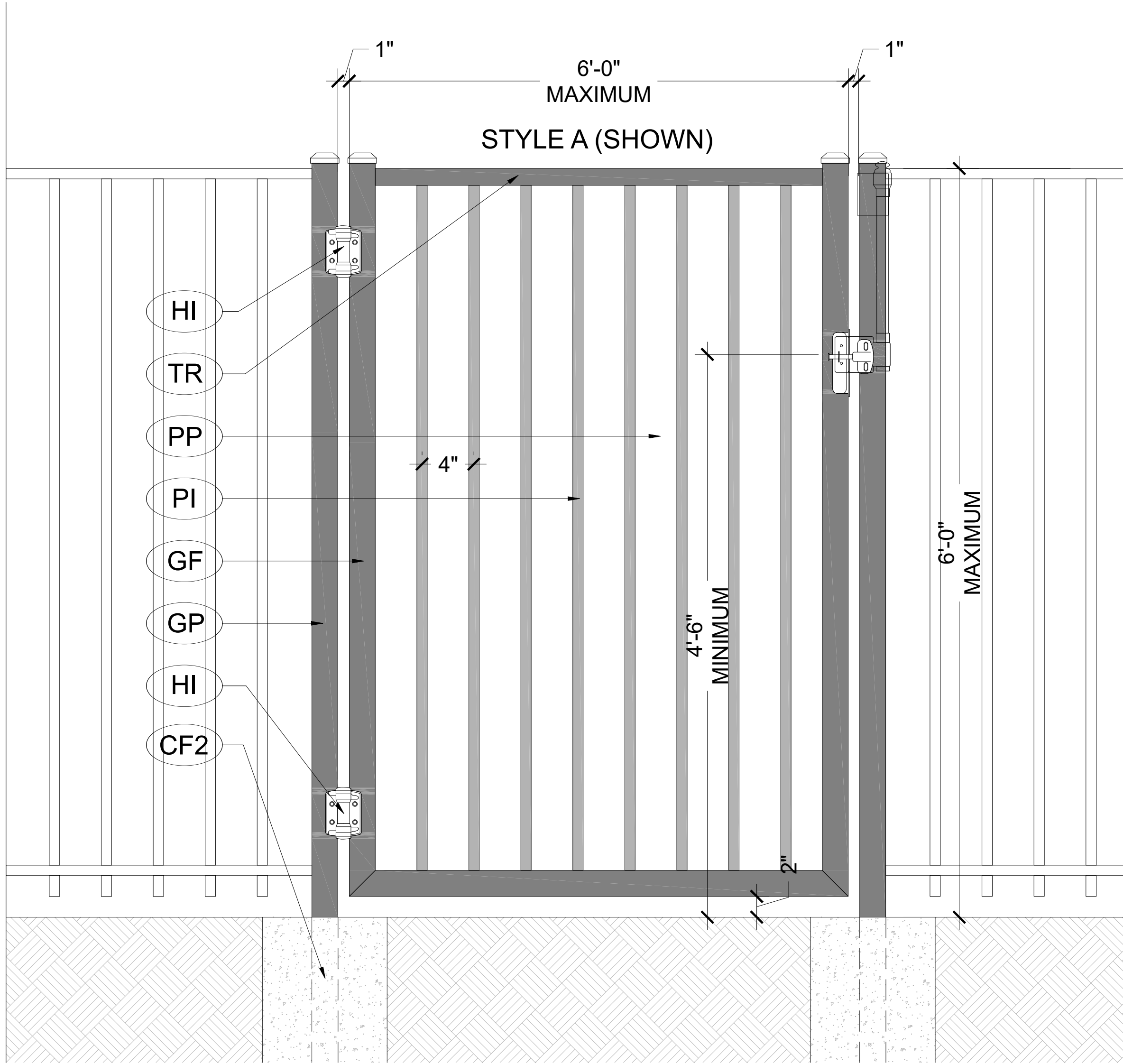
2 SINGLE SWING GATE DETAILS
