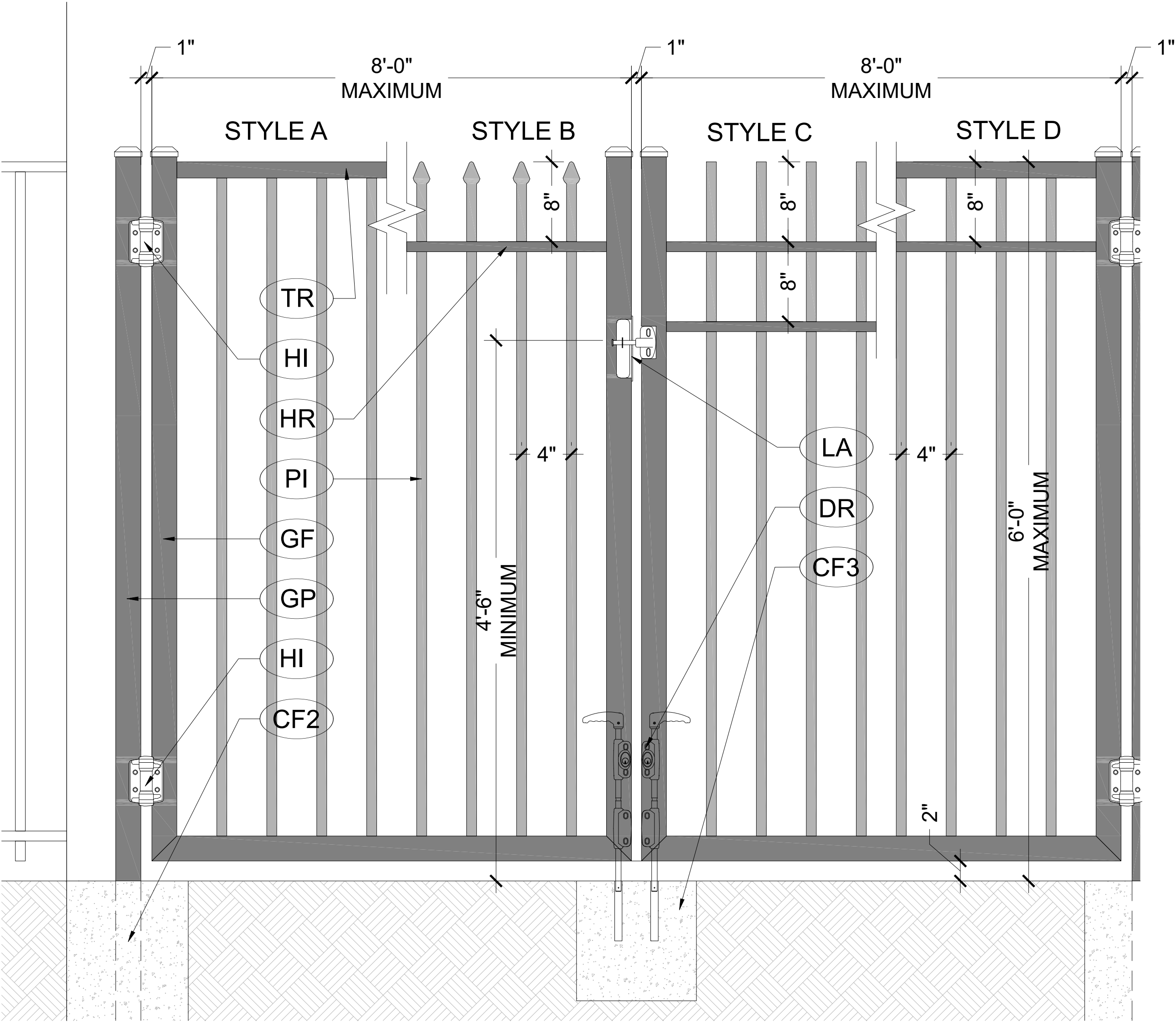
3 DOUBLE SWING GATE DETAILS
