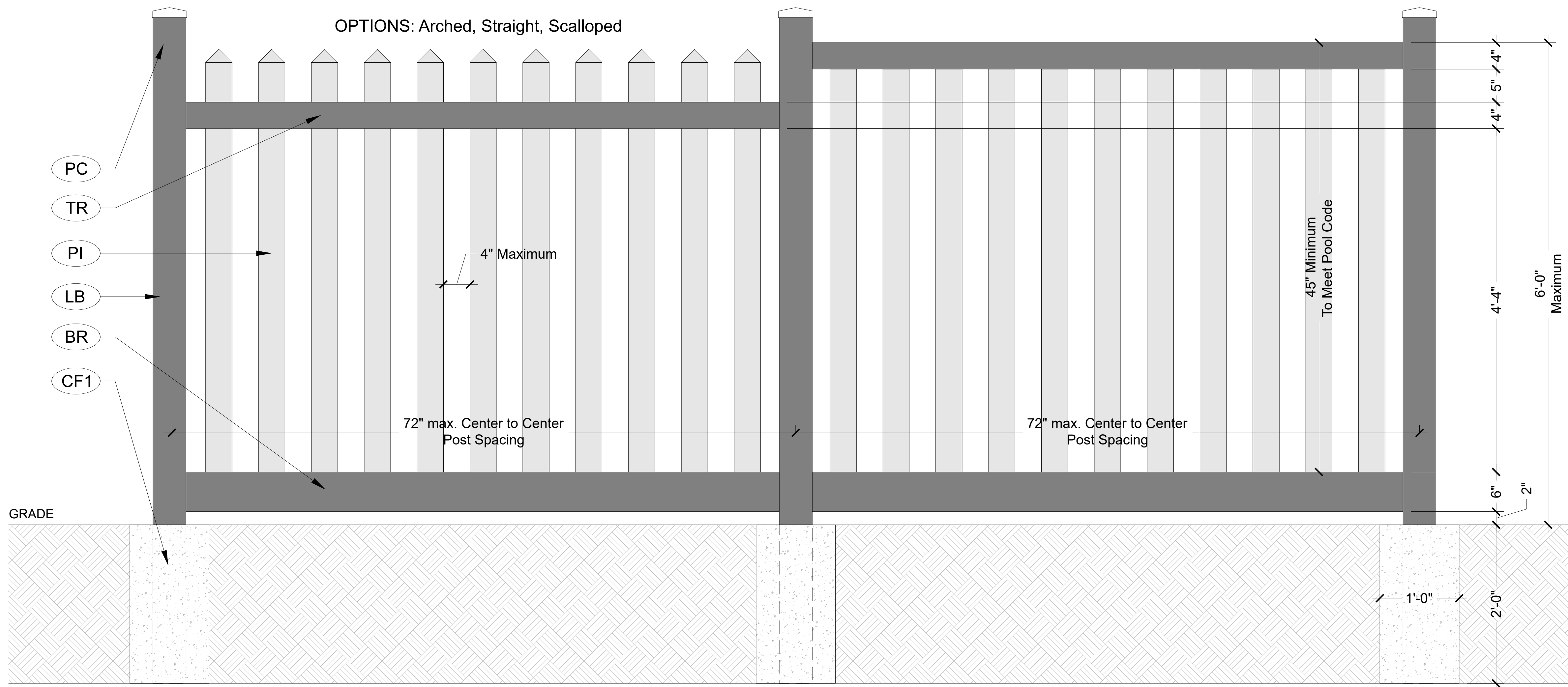
6 Fence Elevation SCALE: 1/2"=1'-0"
