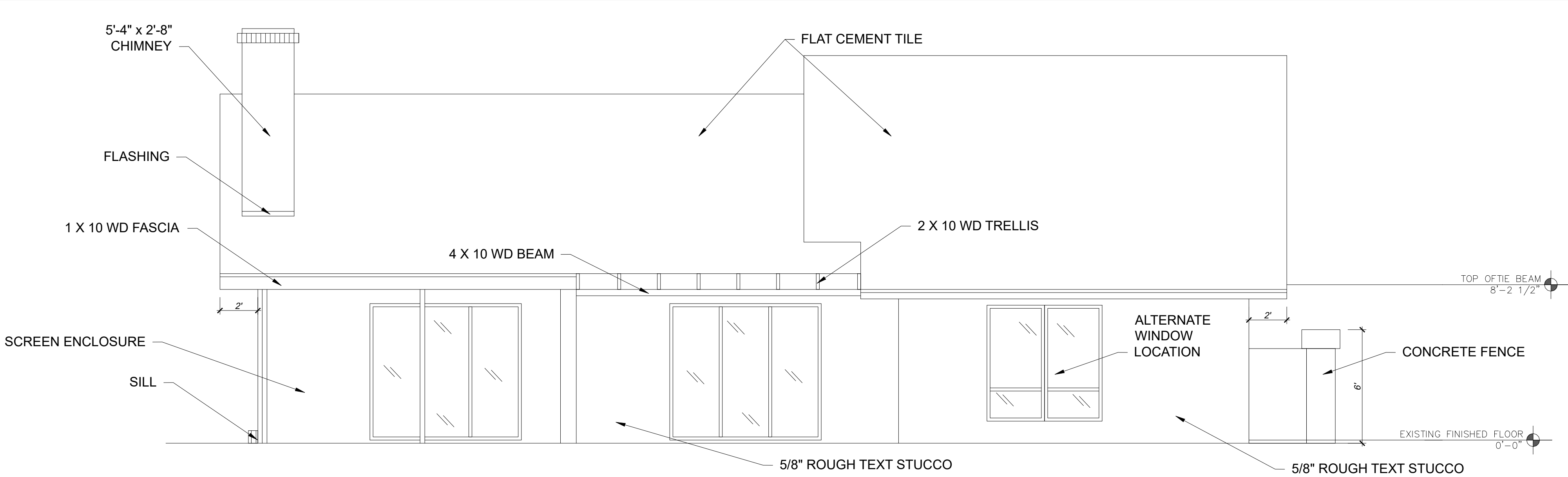
REAR ELEVATION 3/16" = 1'-0"
