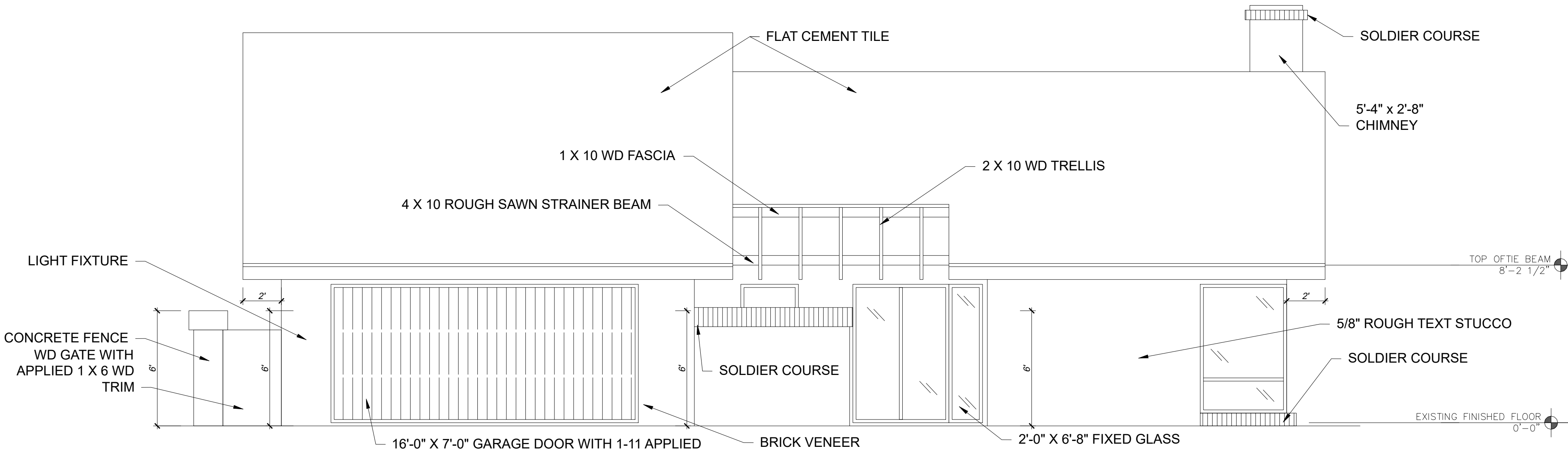
FRONT ELEVATION 3/16" = 1'-0"
