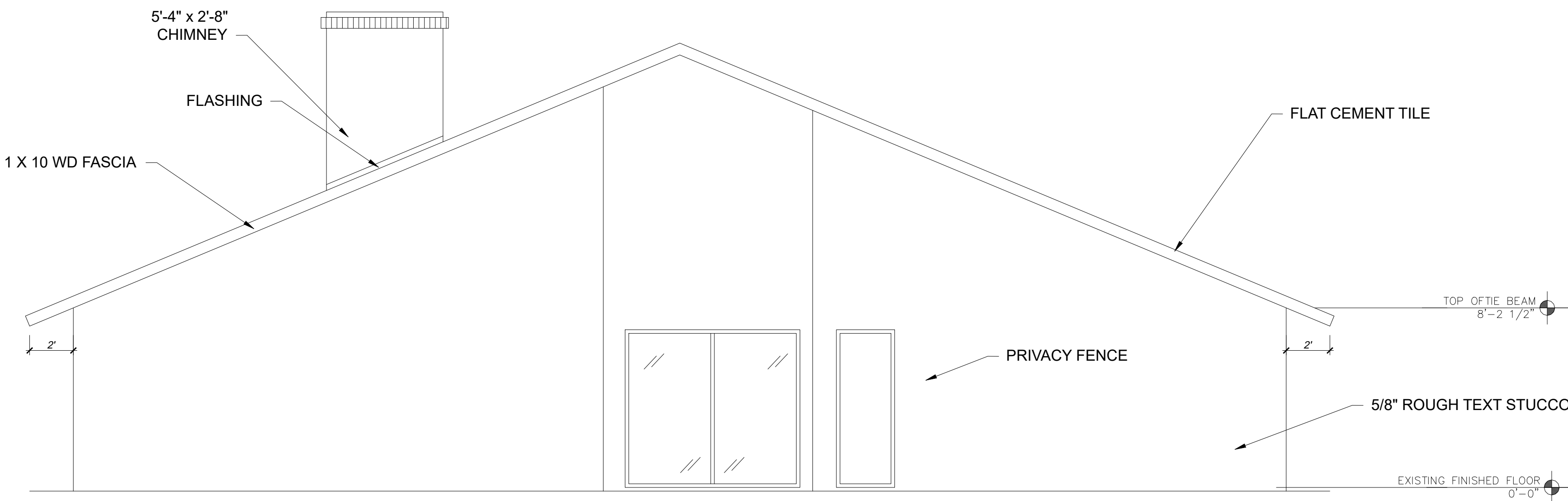
LEFT SIDE ELEVATION 3/16" = 1'-0"
