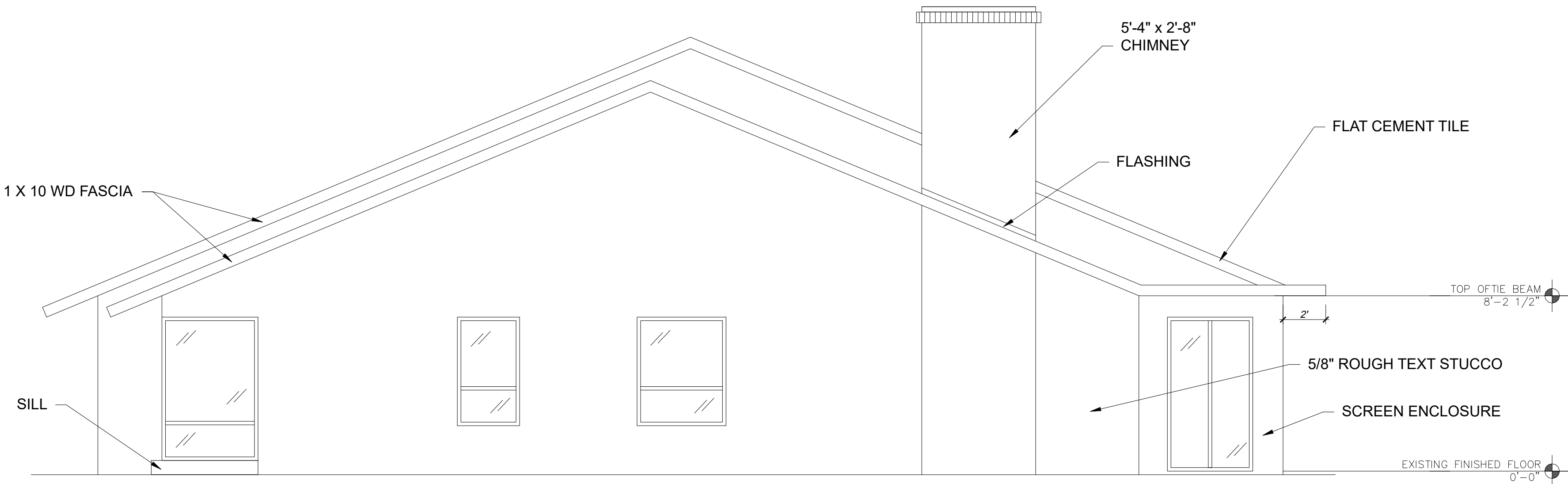
RIGHT SIDE ELEVATION 3/16" = 1'-0"
