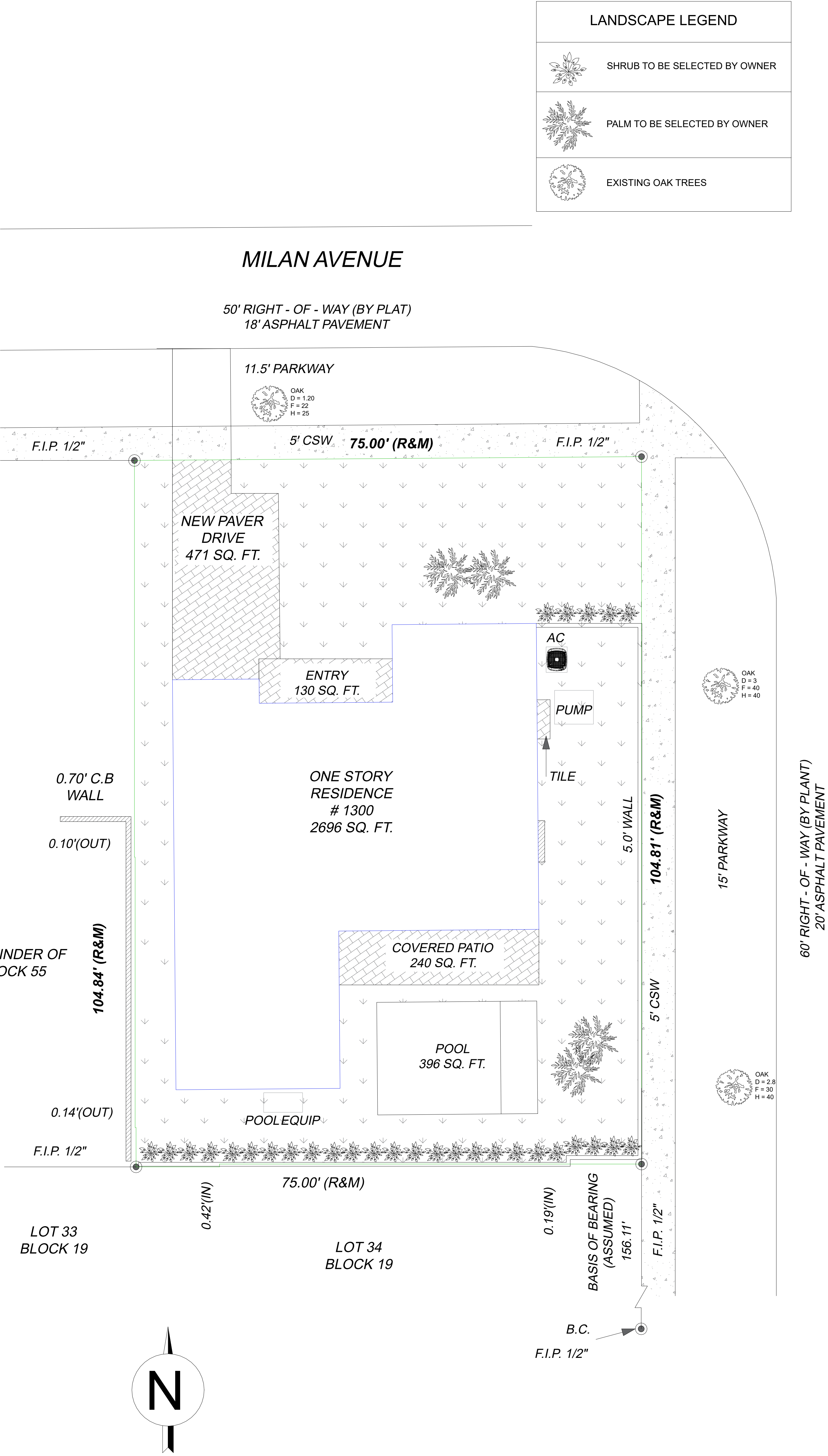
LANDSCAPE PLAN 3/32" = 1'-0"
