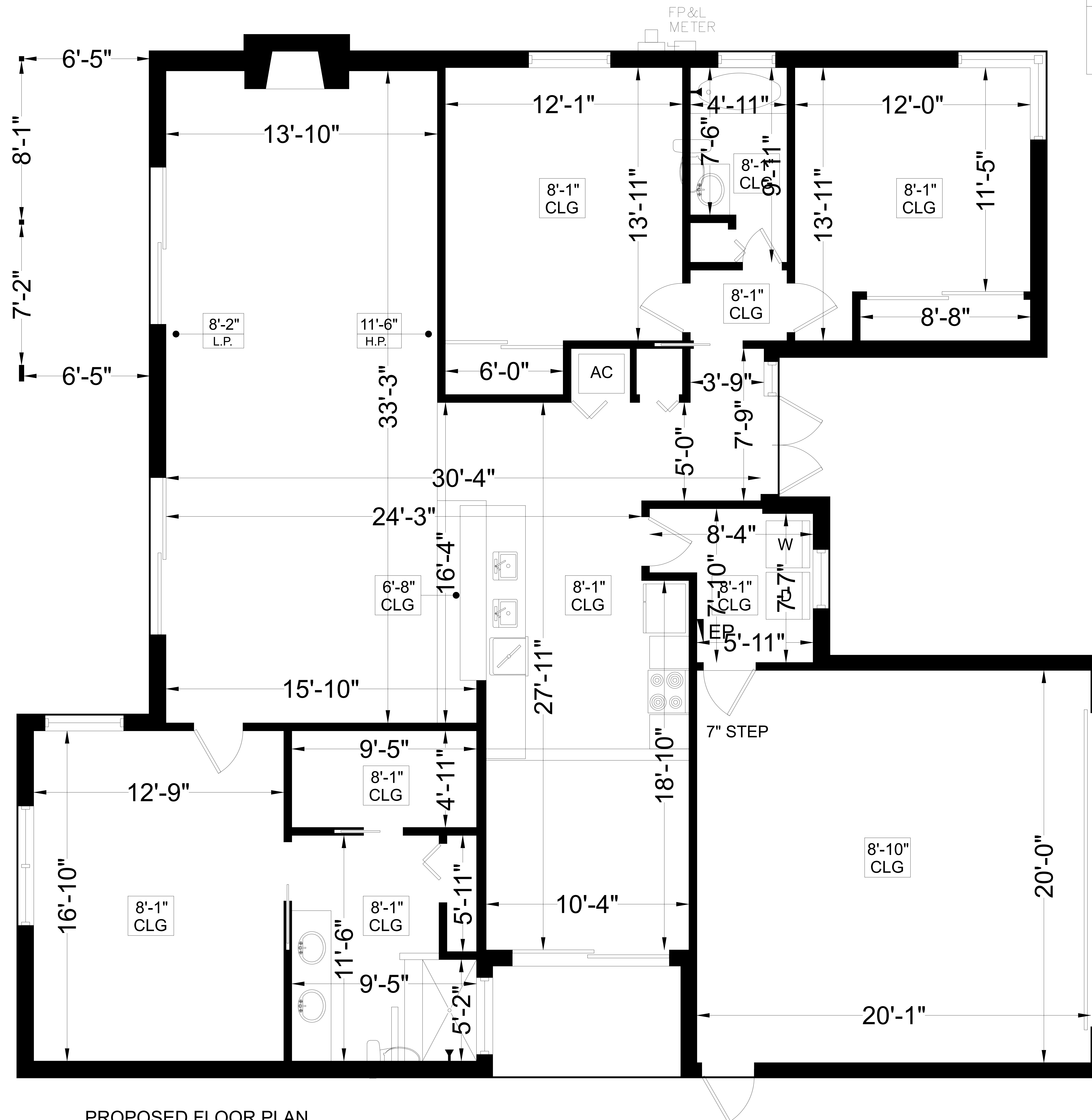
PROPOSED FLOOR PLAN 3/8" = 1'-0"
