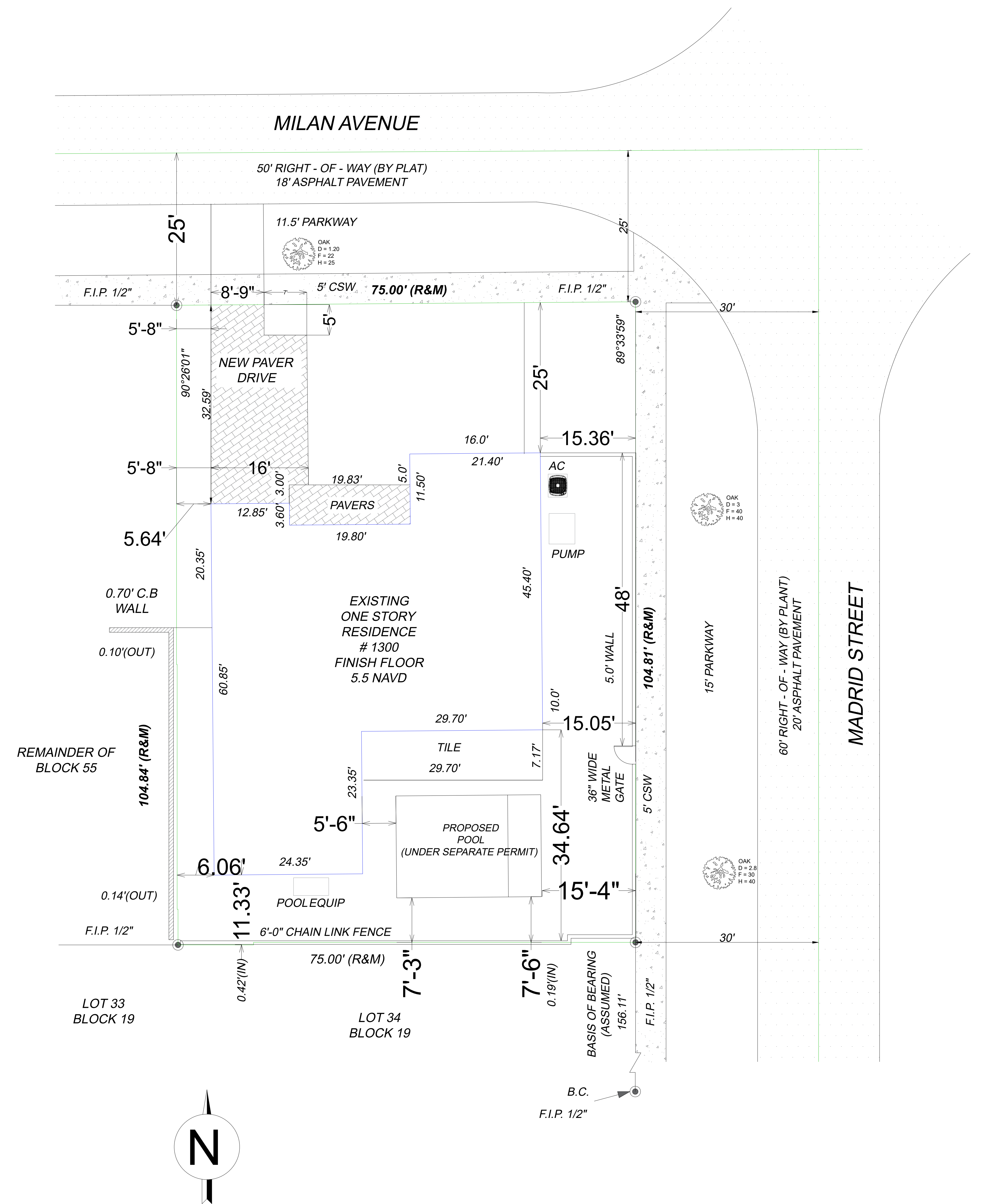
PROPOSED SITE PLAN 3/32" = 1'-0"
