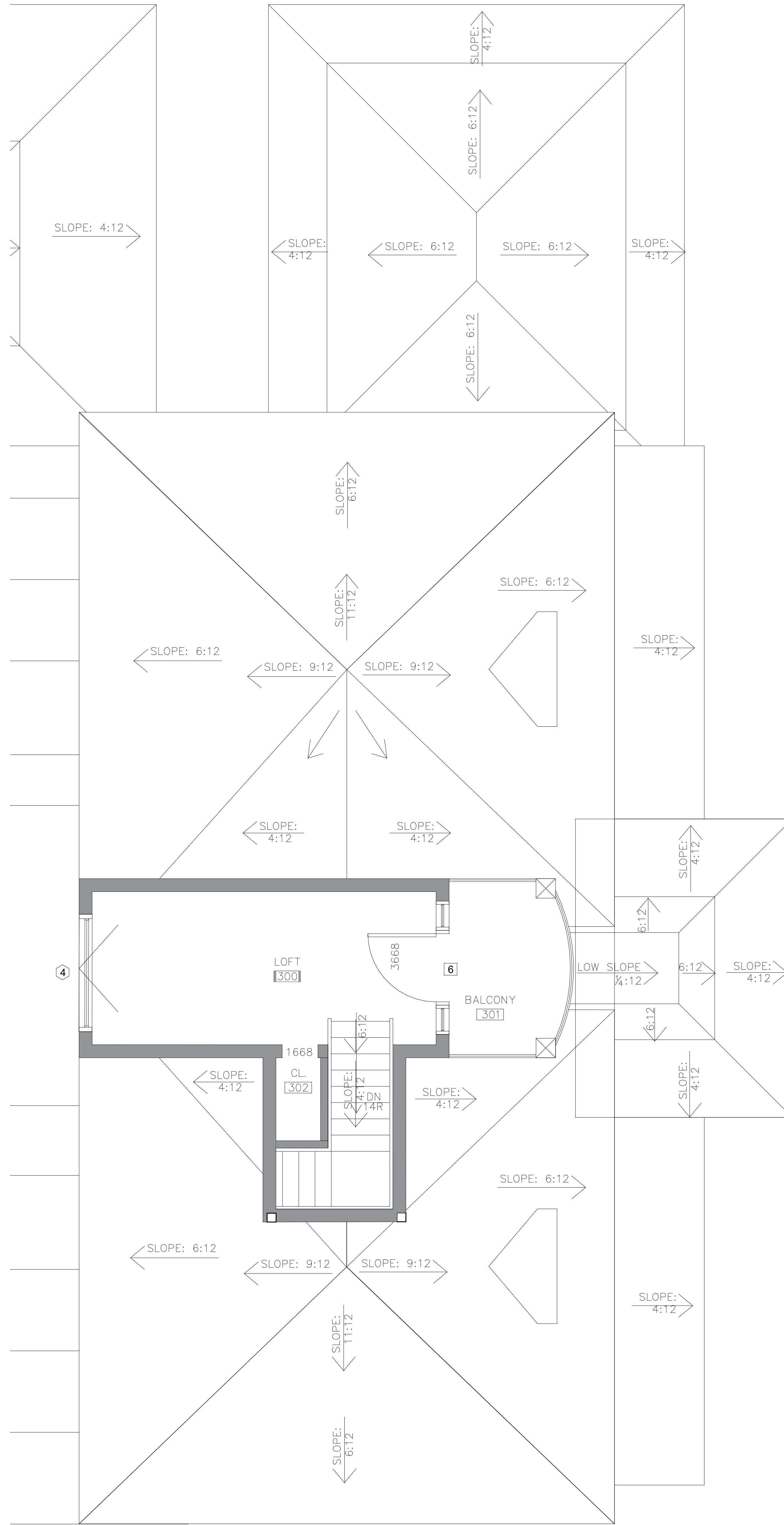
2 PROPOSED LOFT PLAN & SECOND FLOOR ROOF PLAN 1/4" = 1'-0"
