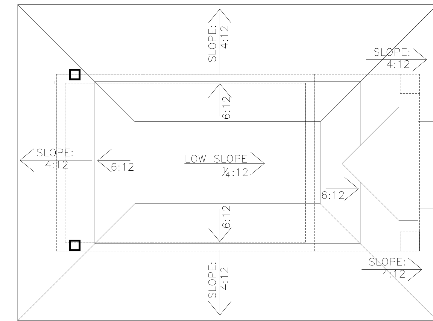
2 PROPOSED LOFT ROOF PLAN 1/4" = 1'-0"
