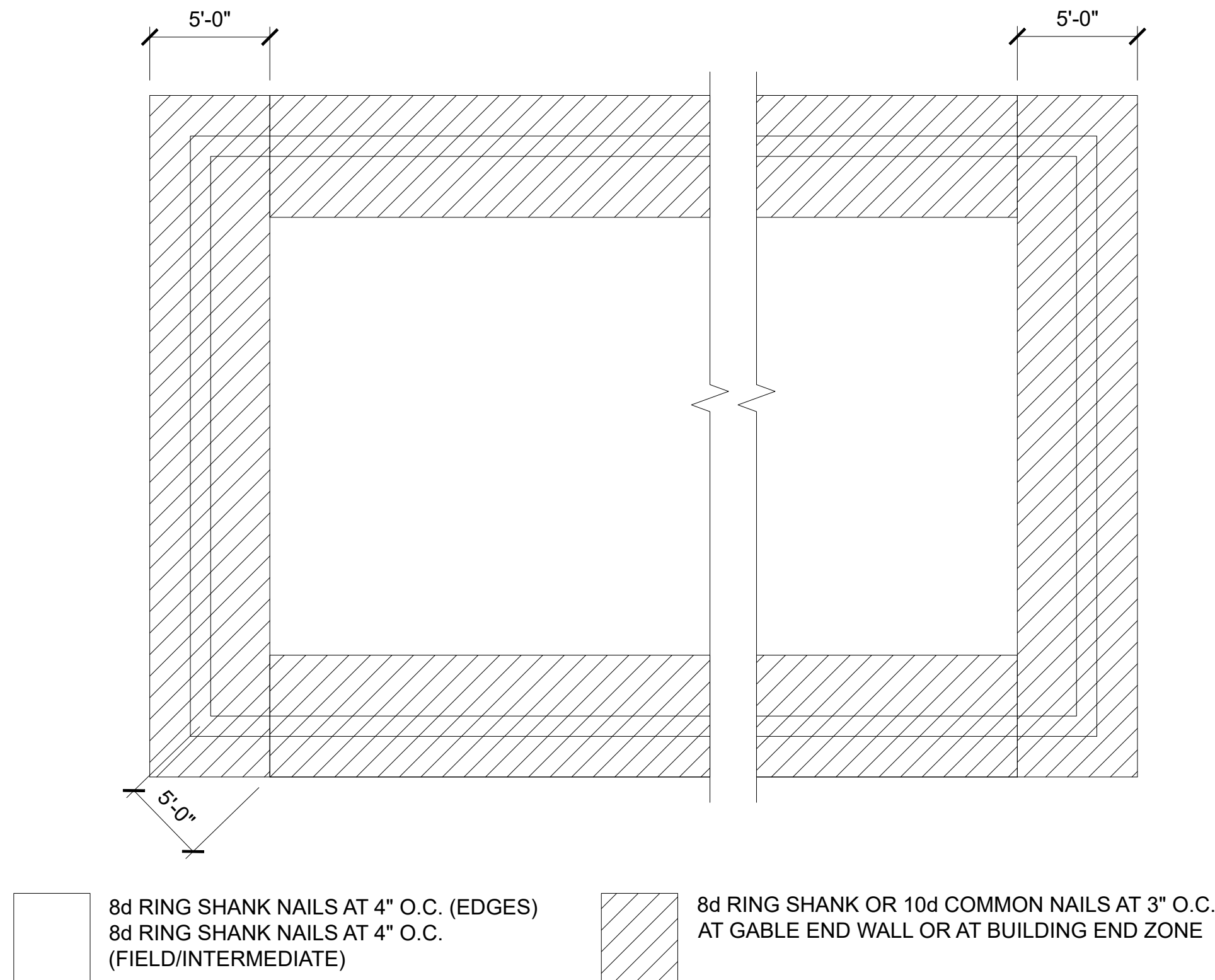
1 ROOF NAILING DETAIL SCALE: 3/4"=1'-0"
