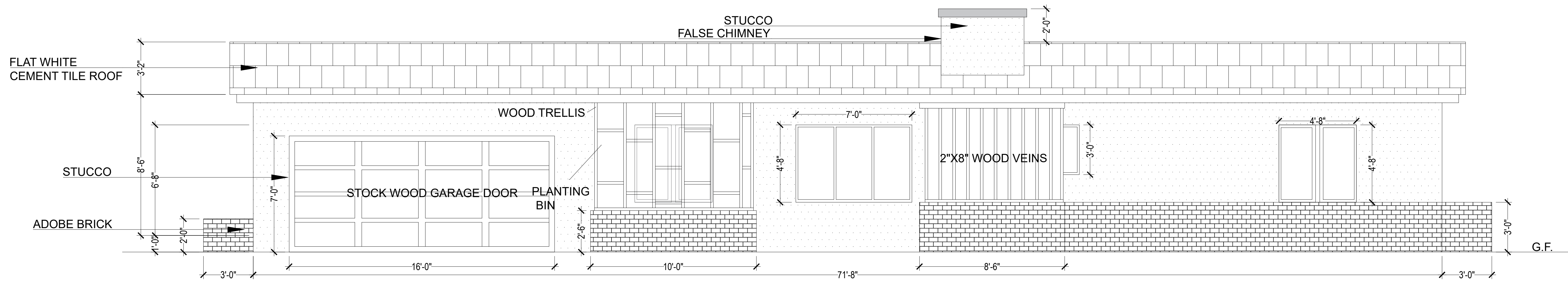
1 FRONT ELEVATION 1/4" = 1'-0"
