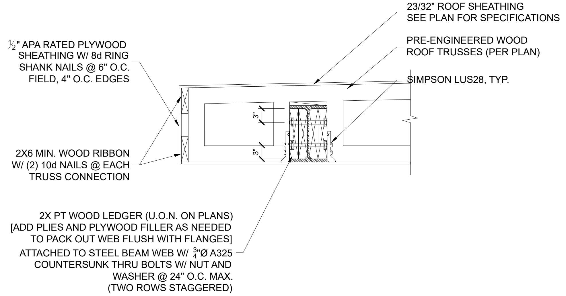
8 SECTION AT ROOF SCALE: 3/4"=1'-0"
