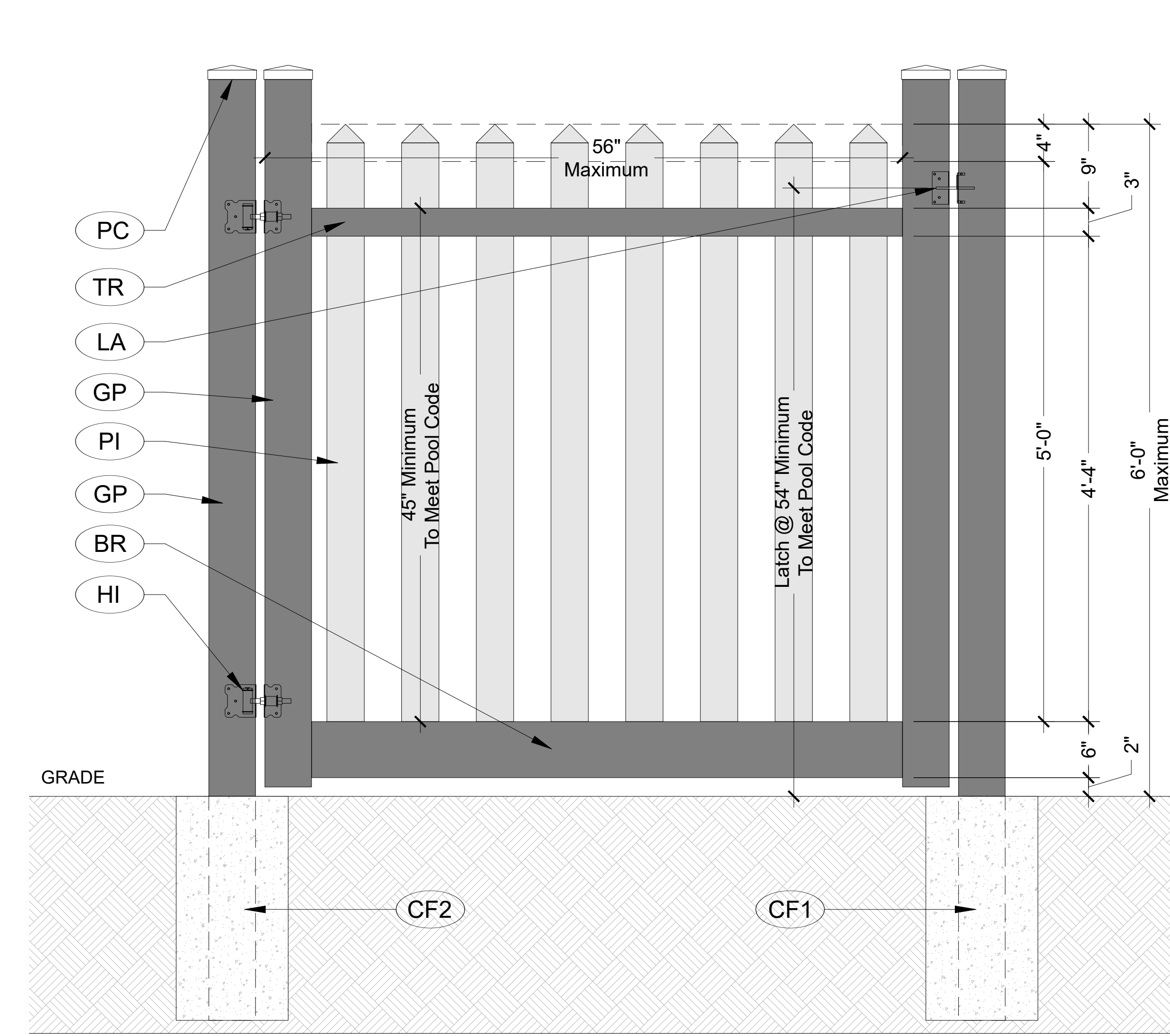
3 Gate DEtails SCALE: 1/2"=1'-0"
