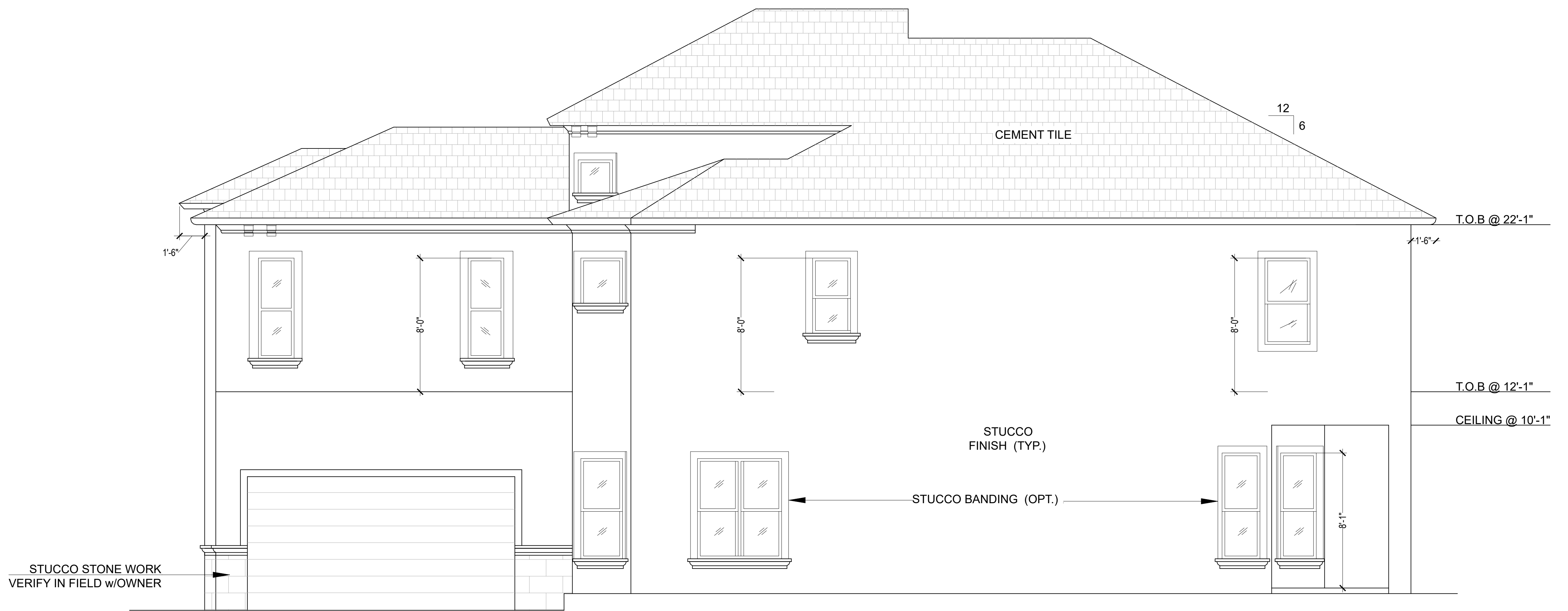
③ RIGHT SIDE ELEVATION 1/4" = 1'-0"
