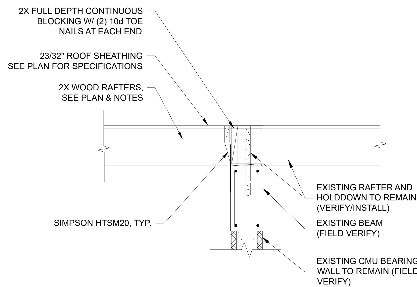
7 NEW RAFTER TO CMU DETAIL SCALE: 3/4"=1'-0"
