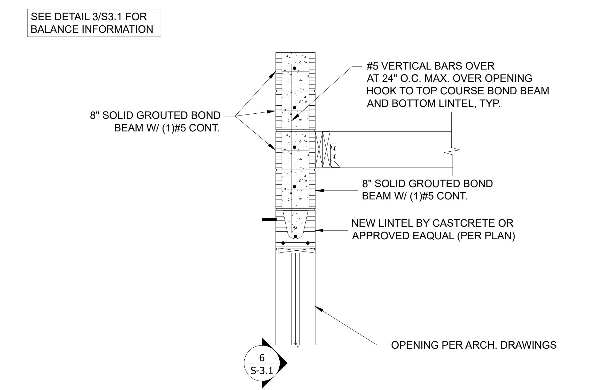
4 SECTION @ OPENING SCALE: 3/4"=1'-0"
