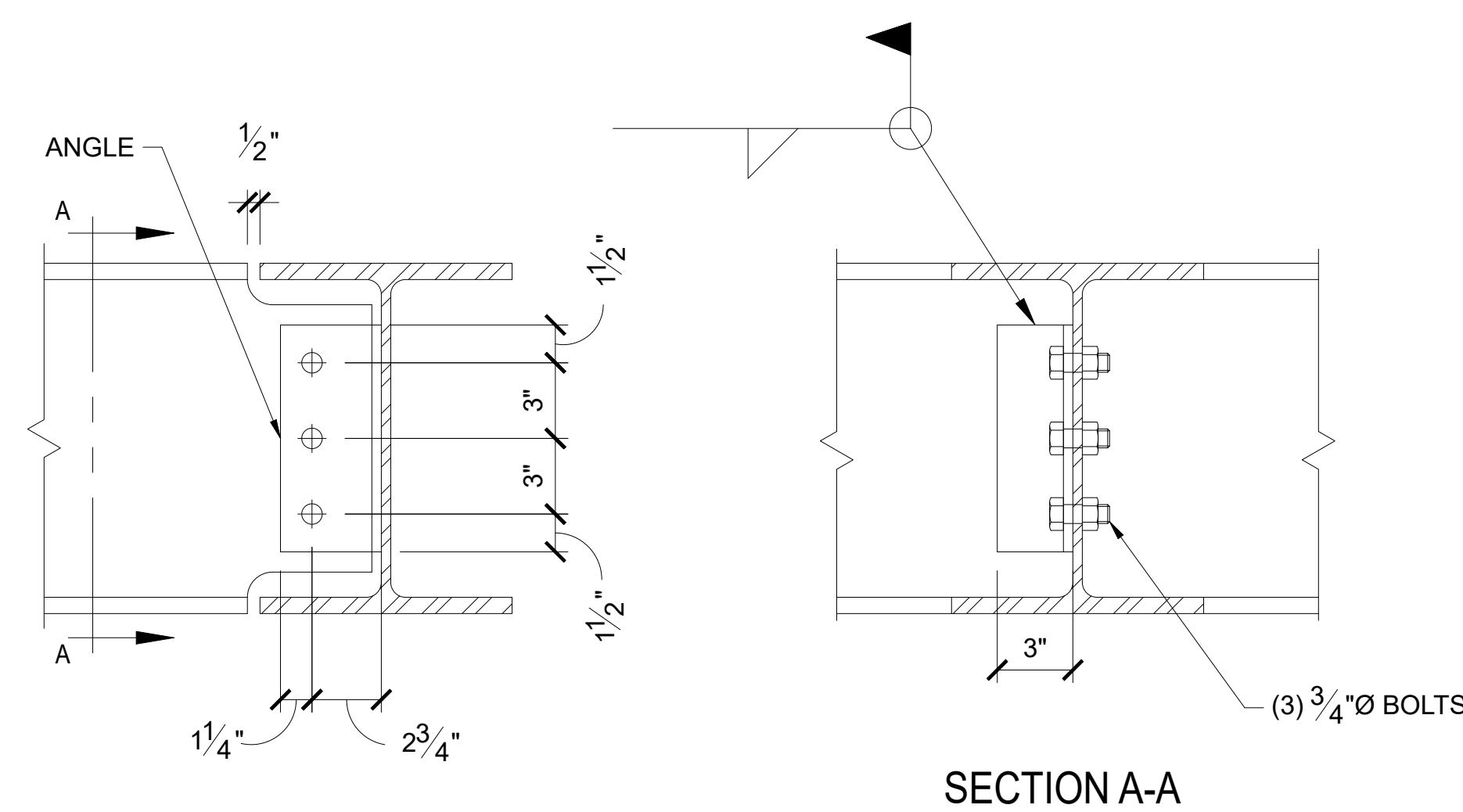
10 STEEL BEAM TO STEEL BEAM CONNECTION SCALE: 1 1/2"=1'-0"
