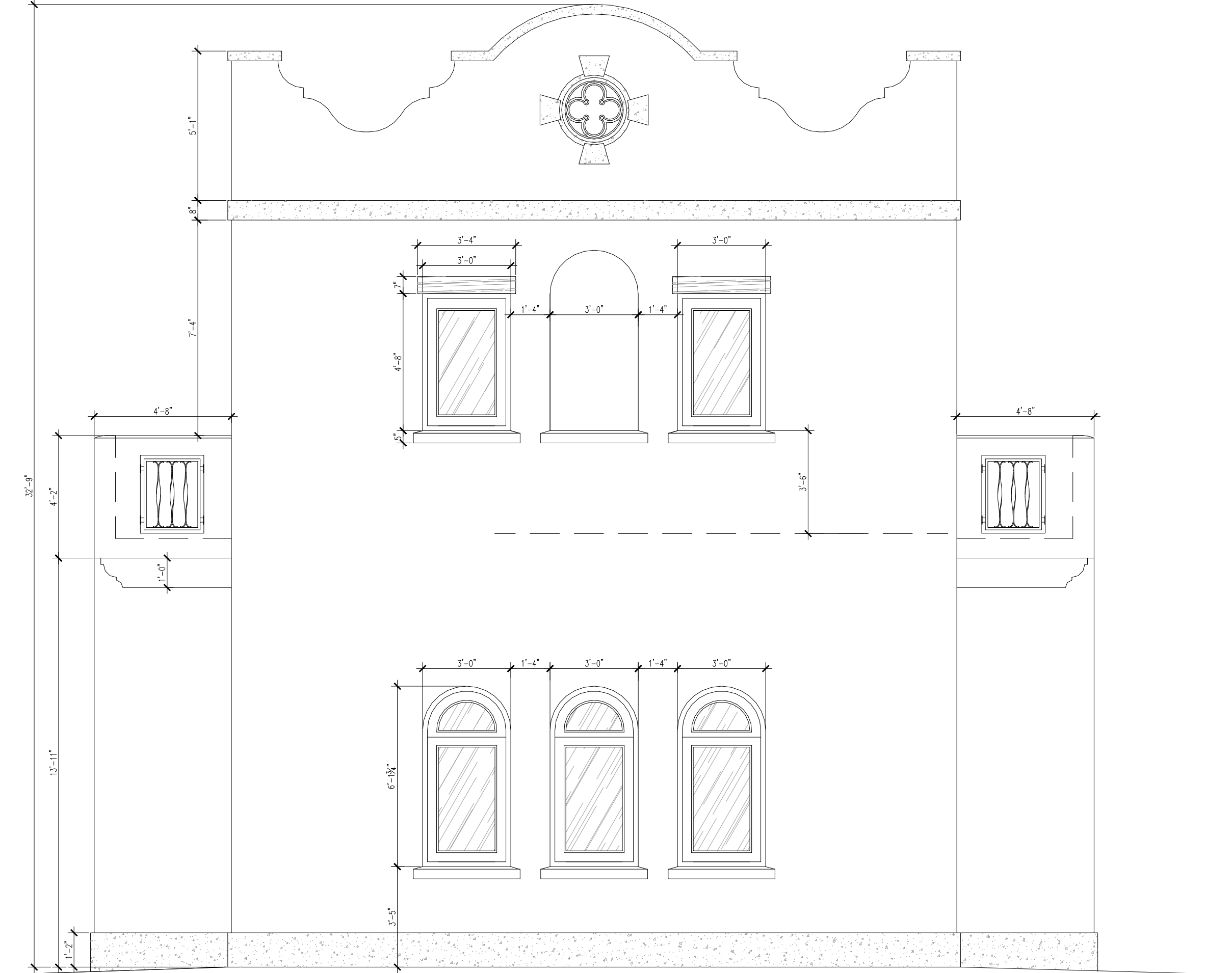
2 WEST ELEVATION 1/4" = 1'-0"
