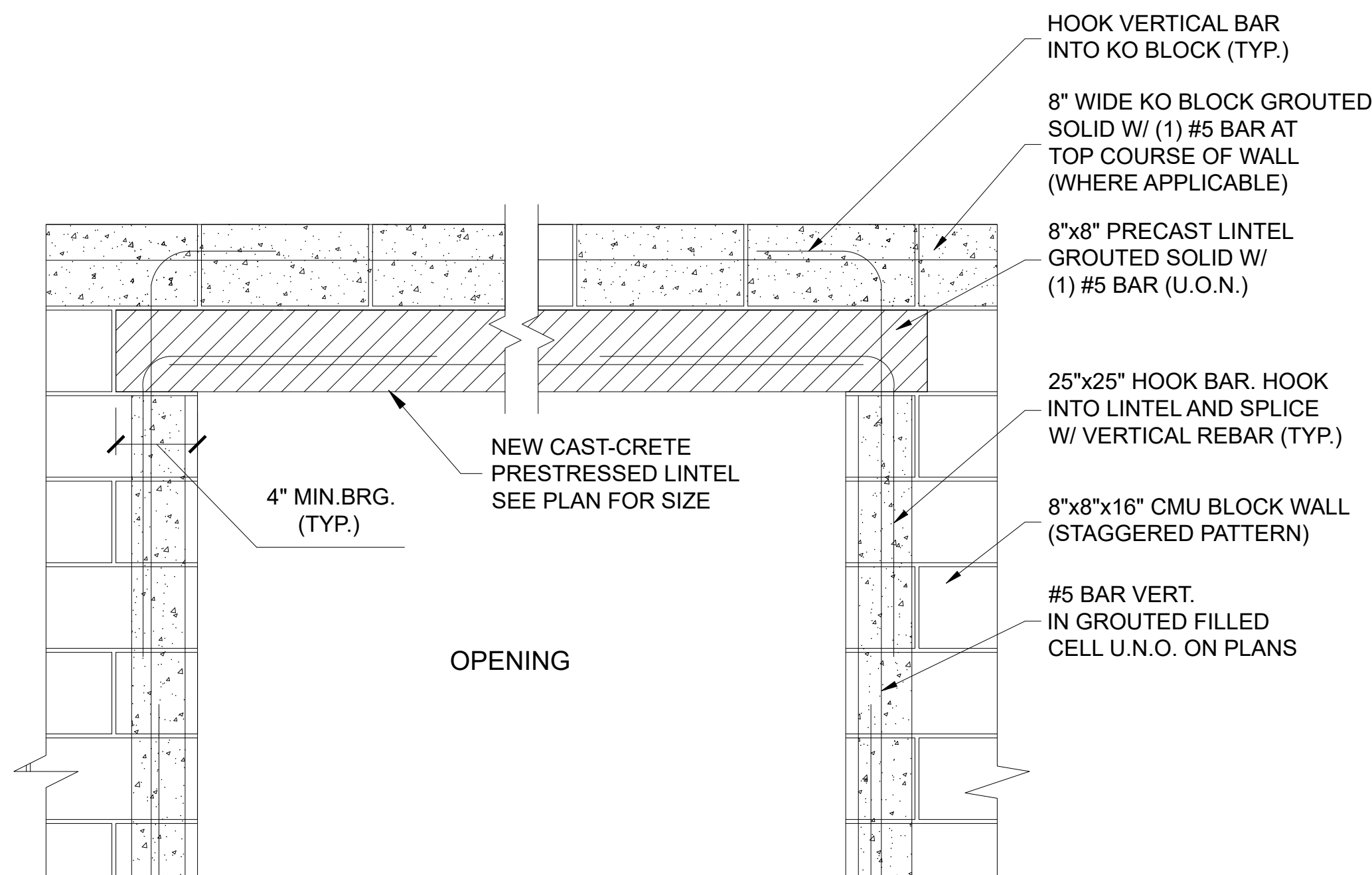
6 TYPICAL LINTEL ASSEMBLY SCALE: 3/4"=1'-0"
