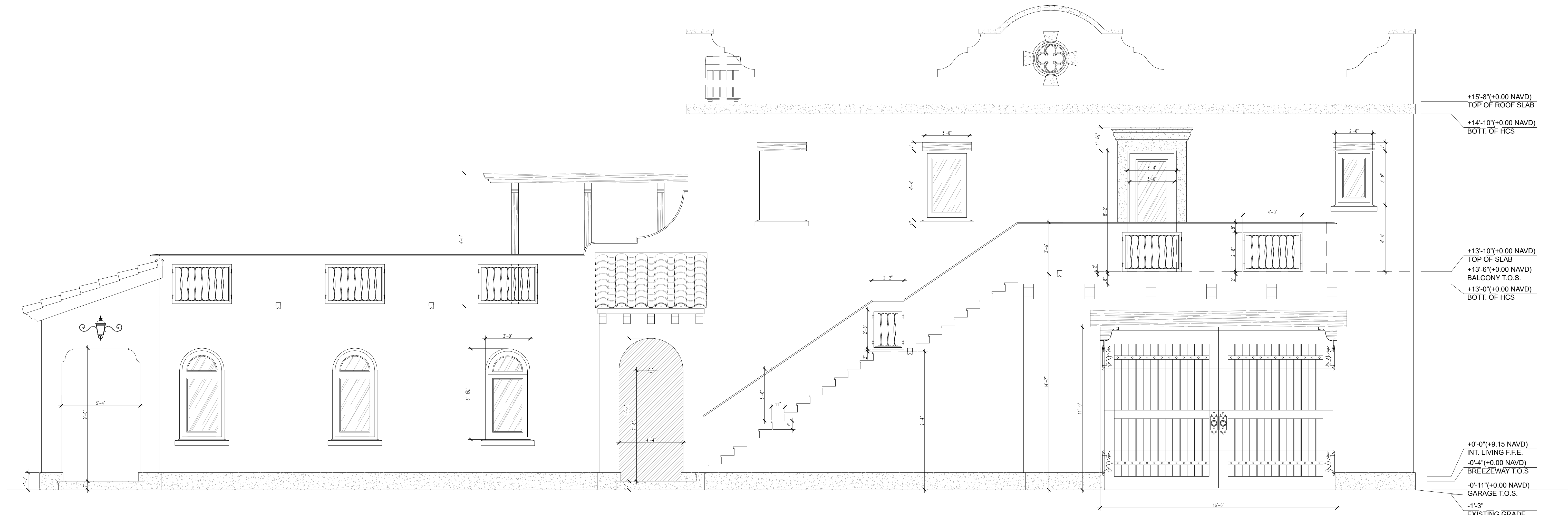
1 NORTH ELEVATION 1/4" = 1'-0"
