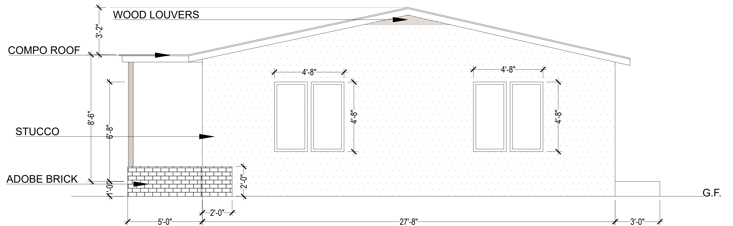
3 RIGHT SIDE ELEVATION 1/4" = 1'-0"
