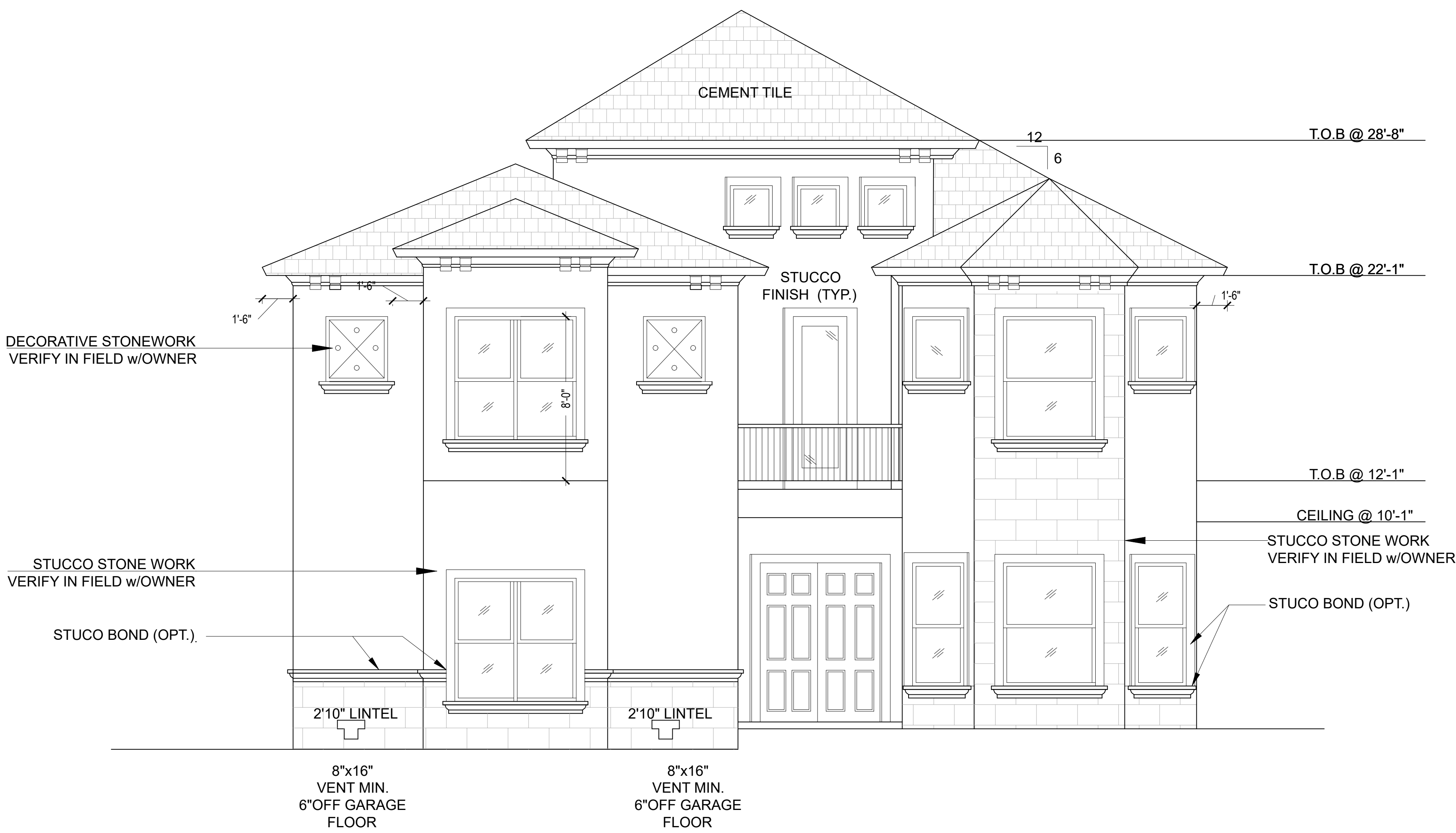
① FRONT ELEVATION 1/4" = 1'-0"
