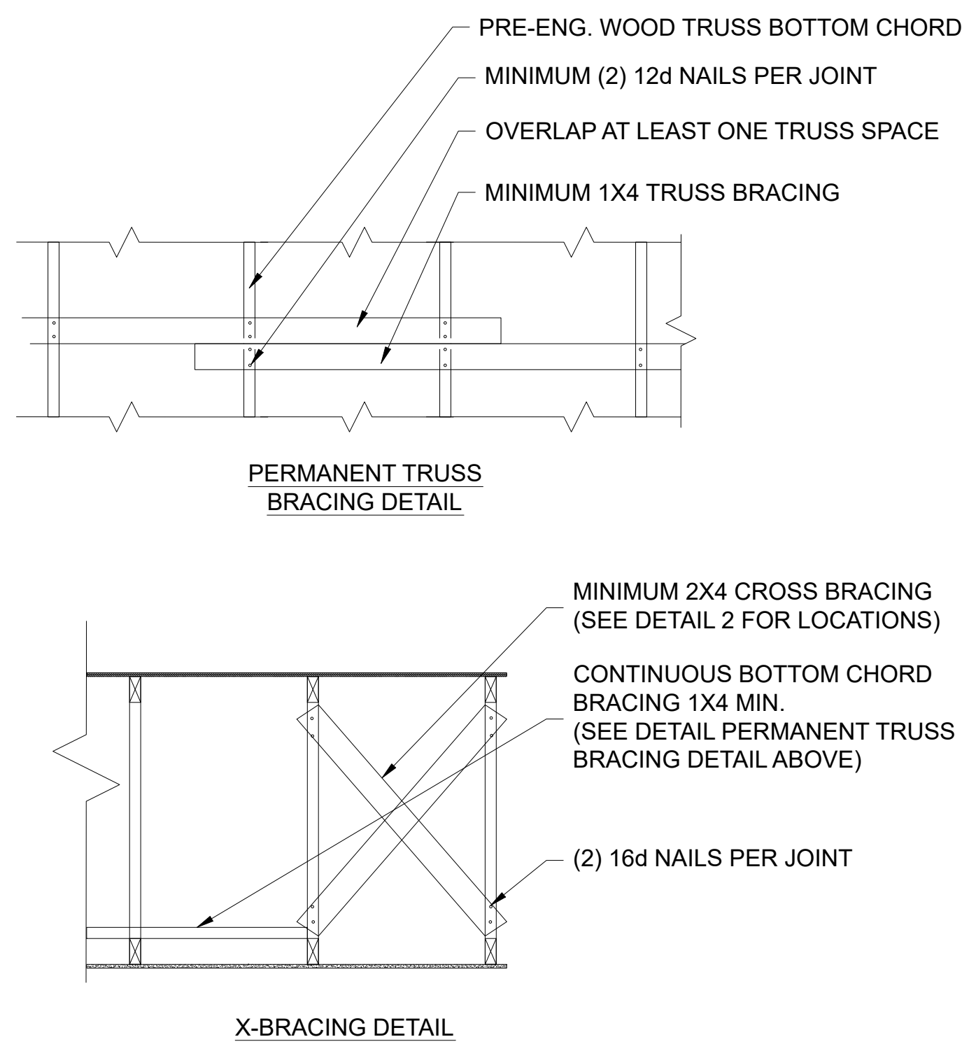
5 ROOF BRACING DETAIL SCALE: 3/4"=1'-0"
