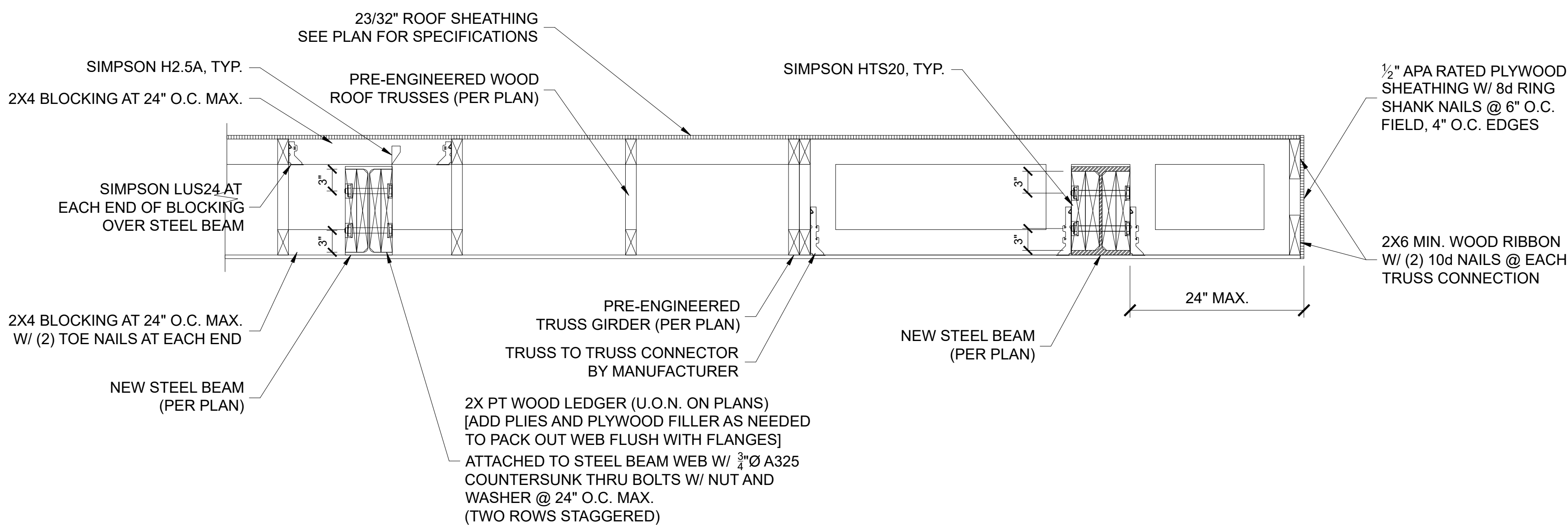
9 NEW ROOF TRUSS AT STEEL BEAM SCALE: 3/4"=1'-0"
