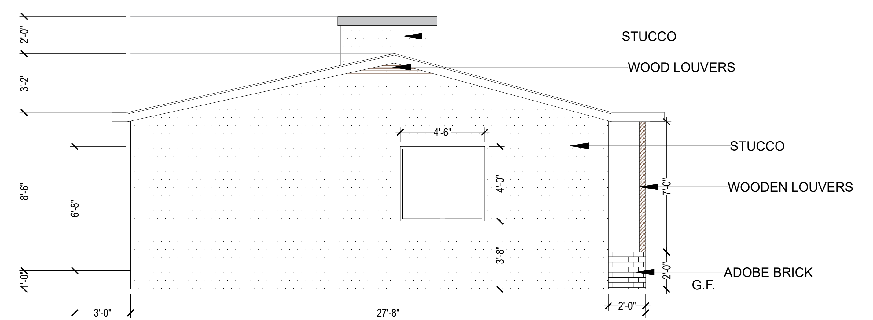
4 LEFT SIDE ELEVATION 1/4" = 1'-0"
