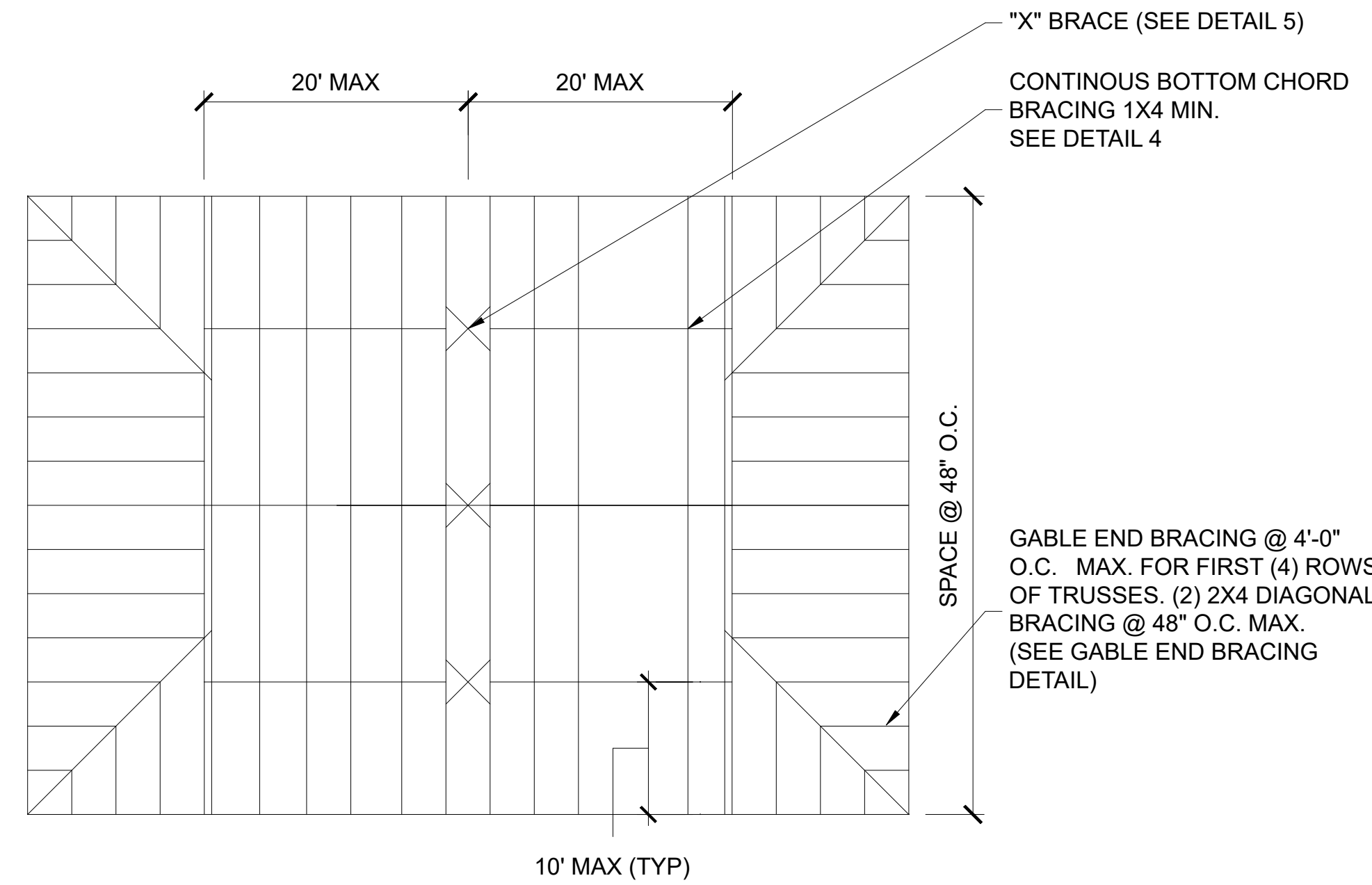
2 ROOF FRAMING DETAIL SCALE: 3/4"=1'-0"
