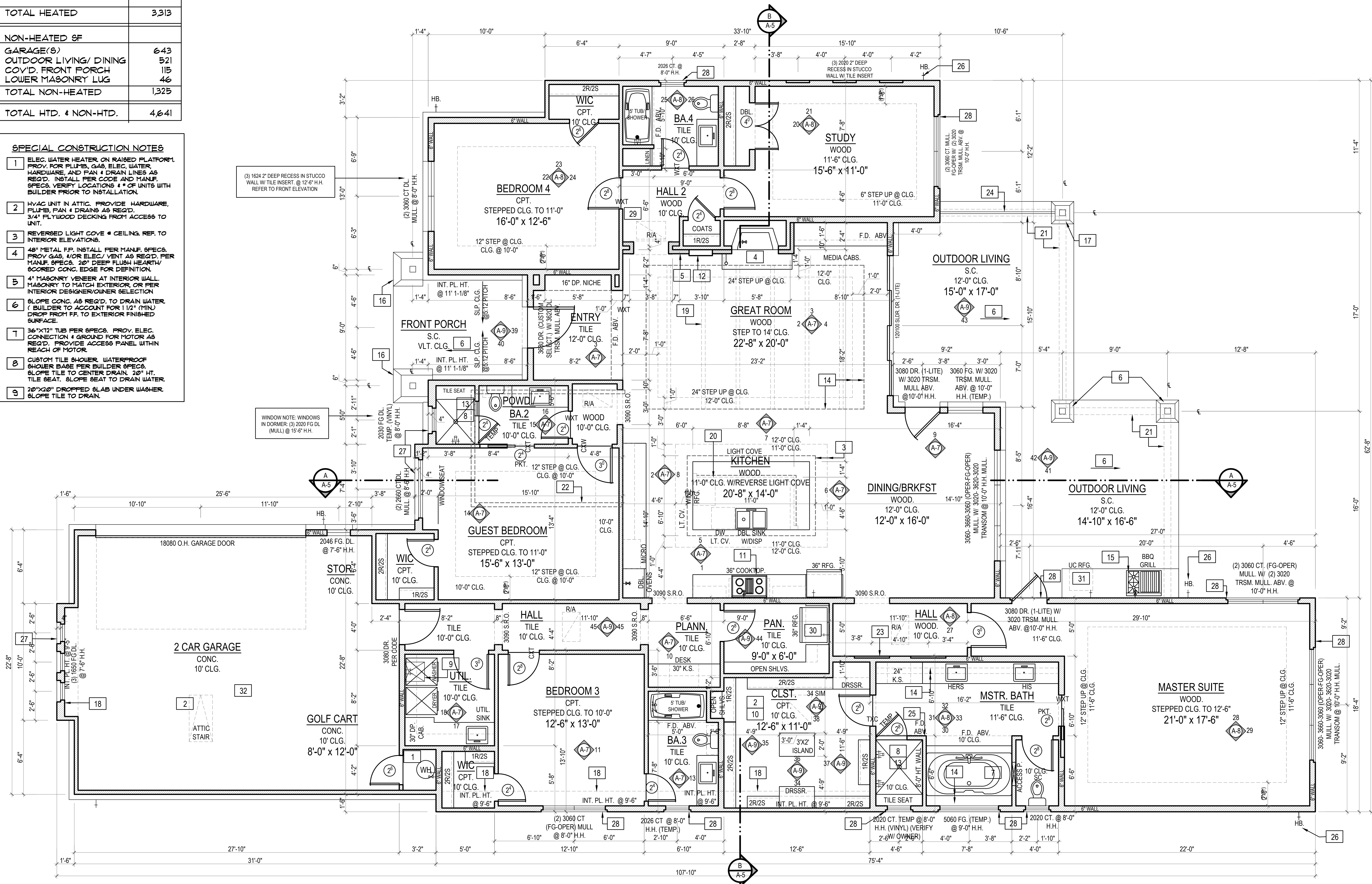
FLOOR PLAN SCALE 1/4" = 1'-0"
