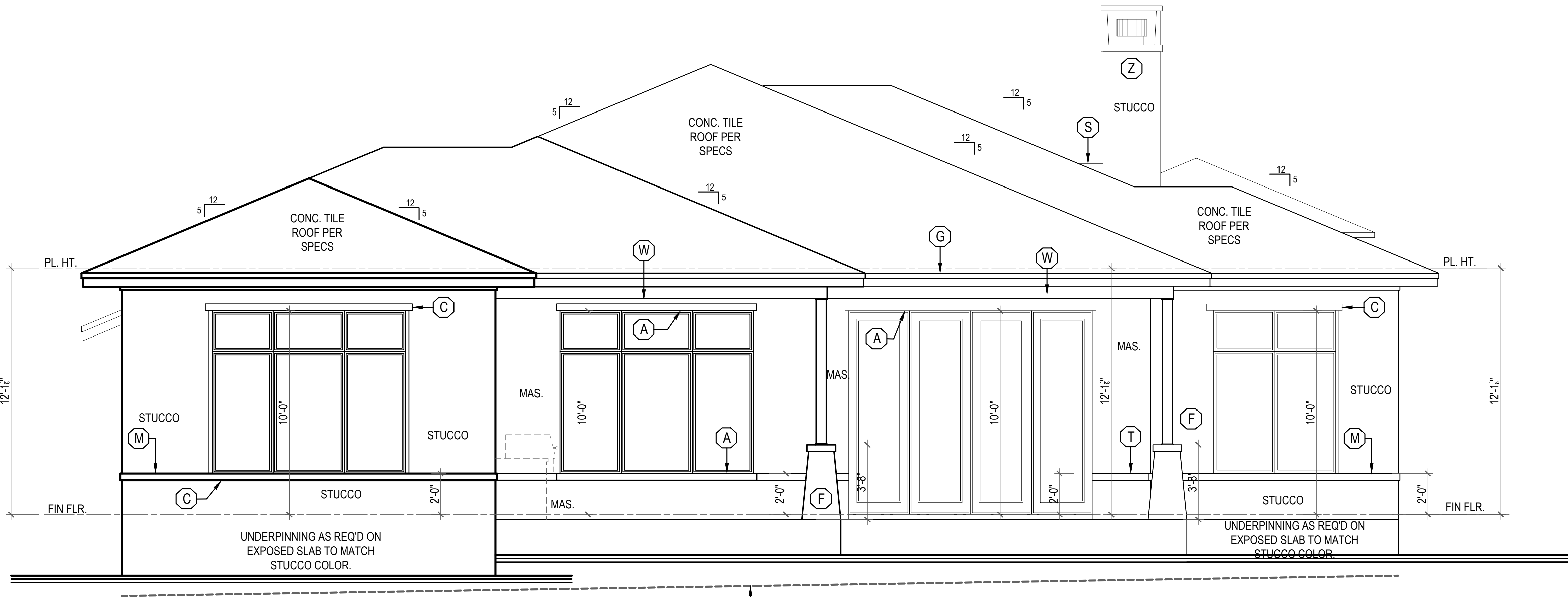
REAR ELEVATION
