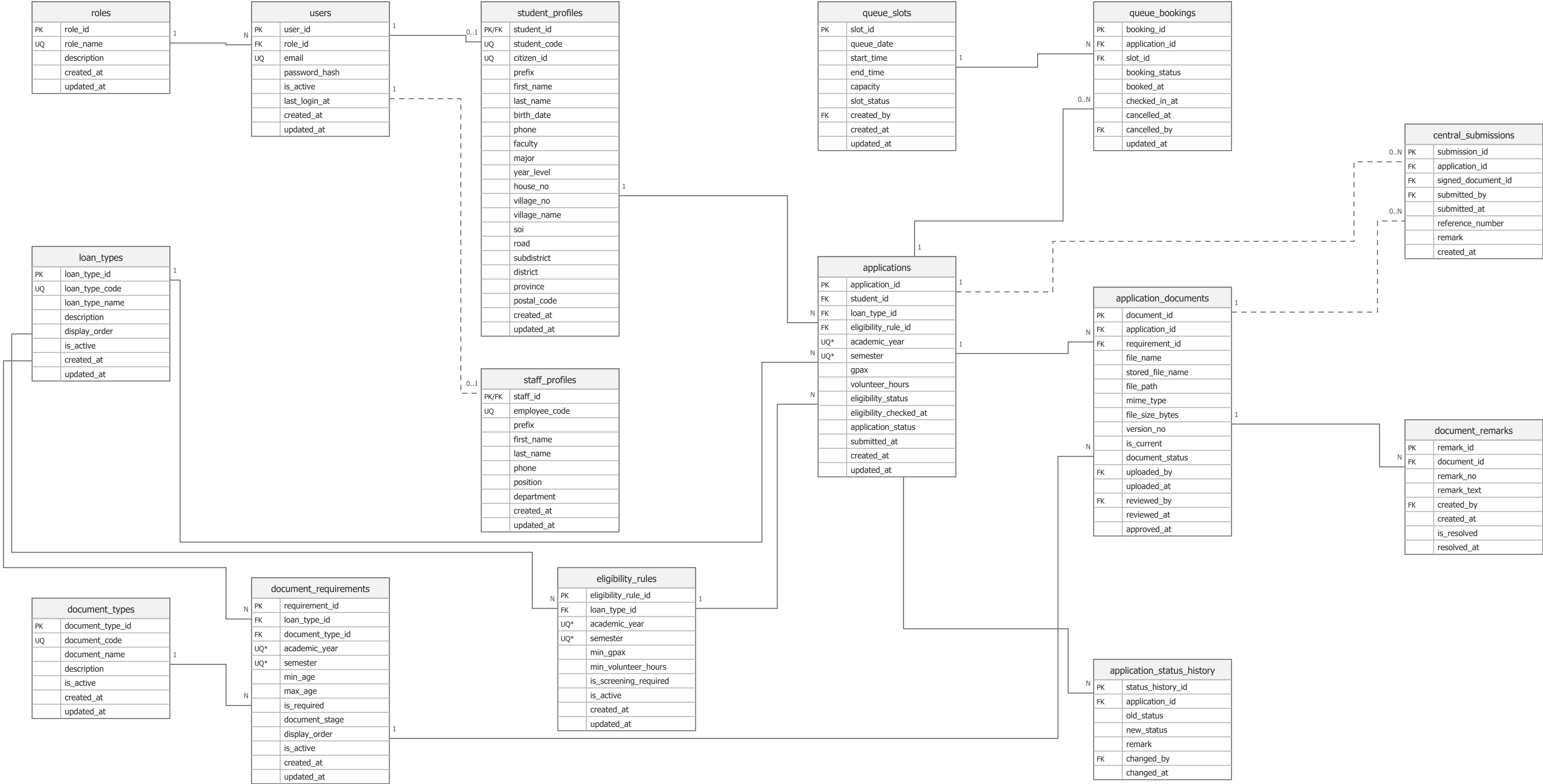
ER Diagram - PSU Student Loan Screening and Queue System
