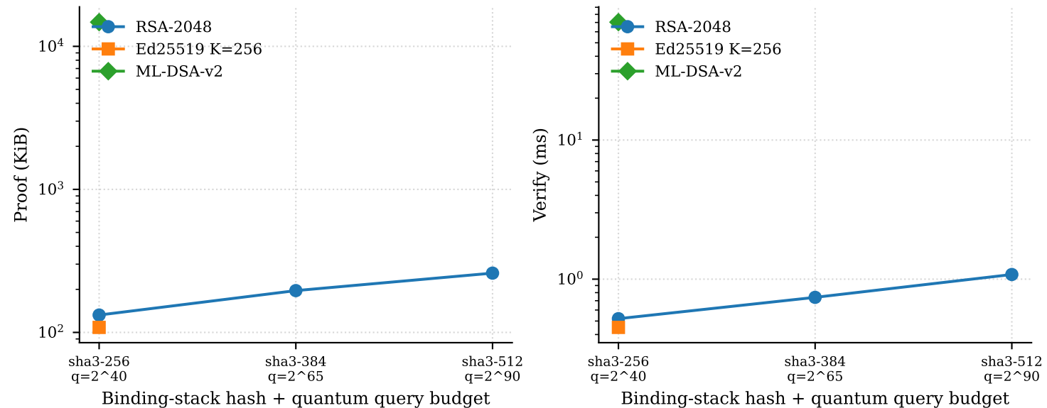
Figure 4. Hash-axis cost progression at L1 — STIR k=2 b=max, \lambda=128 held fixed
