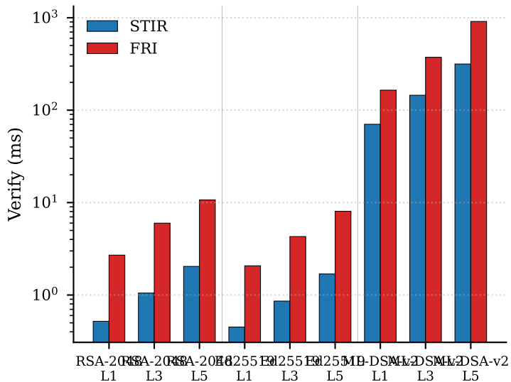
Figure 1. STIR vs FRI at the deployable corner per production AIR Proof size at k=2 , b=\max , q=2^{40} baseline Verify time at k=2 , b=\max , q=2^{40} baseline
