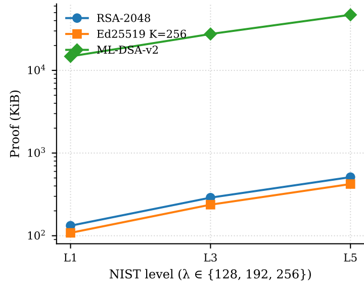
Figure 2. NIST-level cost progression — STIR at k=2 , b=\max Proof size Verify time
